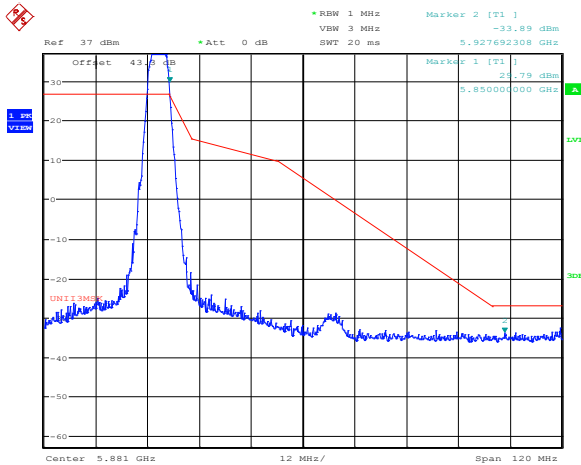
Figure 8.4-81: Conducted upper band edge emissions at 5850 MHz and 5925 MHz, 20 MHz channel, 19 dBi antenna, cho
