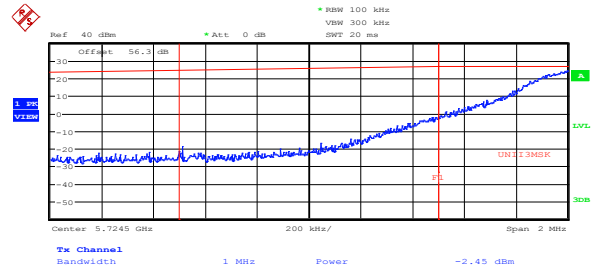
Figure 8.4-41: Conducted lower band edge emissions at 5725 MHz, 5 MHz channel, 32 dBi antenna, cho
