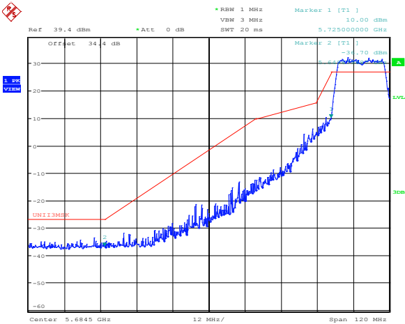
Figure 8.4-60: Conducted lower band edge emissions at 5650 MHz and 5725 MHz, 5 MHz channel, 10 dBi antenna, cho
