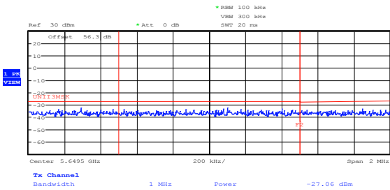
Figure 8.4-42: Conducted lower band edge emissions at 5650 MHz, 10 MHz channel, 32 dBi antenna, cho
