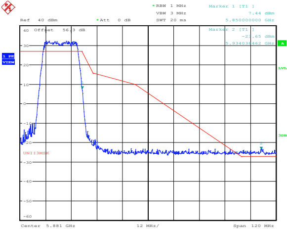
Figure 8.4-68: Conducted upper band edge emissions at 5850 MHz, 10 MHz channel, 32 dBi antenna, cho
