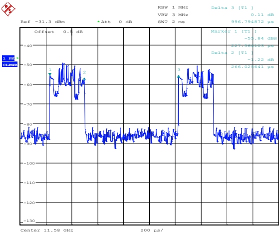
Diagram 8.4-1: Duty cycle for 5 MHz channel
