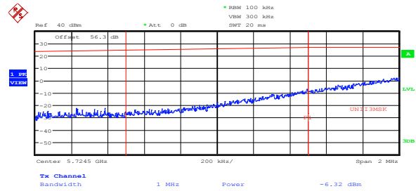
Figure 8.4-43: Conducted lower band edge emissions at 5725 MHz, 10 MHz channel, 32 dBi antenna, cho
