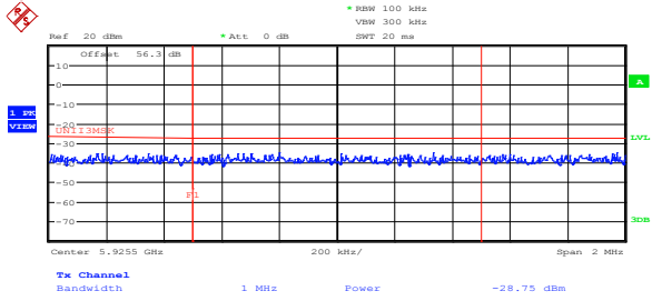
Figure 8.4-69: Conducted upper band edge emissions at 5925 MHz, 10 MHz channel, 32 dBi antenna, cho
