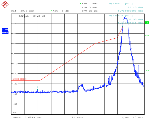
Figure 8.4-61: Conducted lower band edge emissions at 5650 MHz and 5725 MHz, 10 MHz channel, 10 dBi antenna, cho
