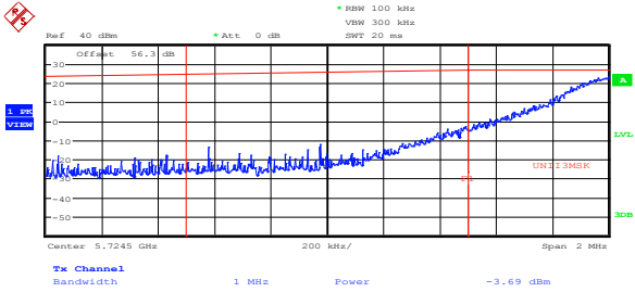
Figure 8.4-45: Conducted lower band edge emissions at 5725 MHz, 20 MHz channel, 32 dBi antenna, cho
