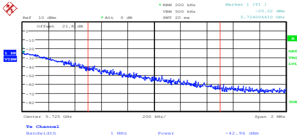
Diagram 8.5-5: Upper band edge sample plot
