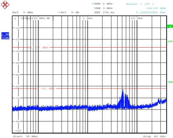
Diagram 8.5-105: Conducted spurious emissions for IC, 32 dBi antenna, 10 MHz channel, ch1, low frequency
