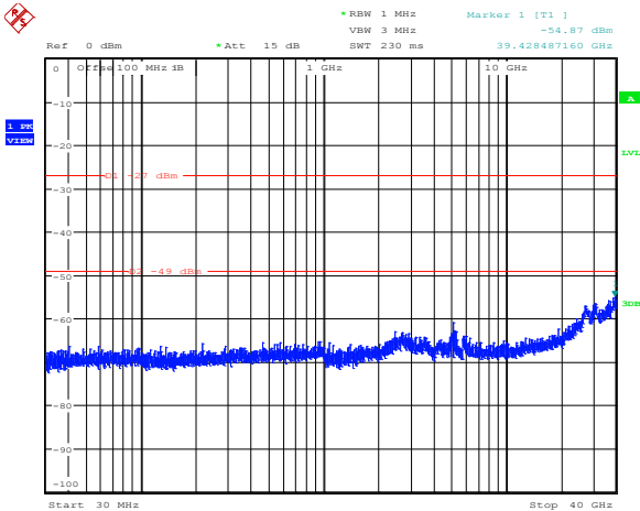
Diagram 8.5-85: Conducted spurious emissions for IC, 19 dBi antenna, 10 MHz channel, cho, mid frequency
