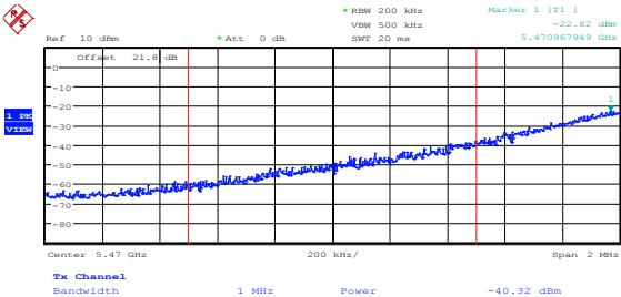
Diagram 8.5-4: Lower band edge sample plot
