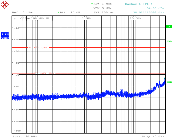
Diagram 8.5-84: Conducted spurious emissions for IC, 19 dBi antenna, 10 MHz channel, cho, low frequency
