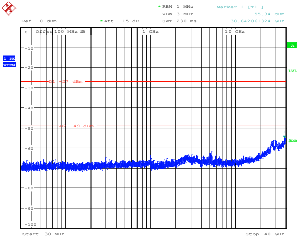
Diagram 8.5-23: Conducted spurious emissions for FCC, 10 dBi antenna, 20 MHz channel, ch1, high frequency
