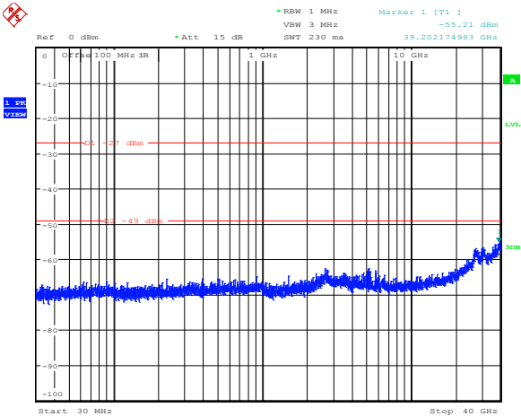
Diagram 8.5-26: Conducted spurious emissions for FCC, 19 dBi antenna, 5 MHz channel, cho, high frequency
