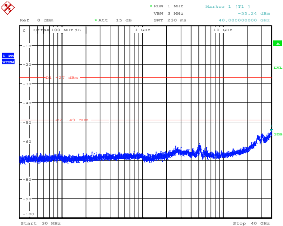
Diagram 8.5-38: Conducted spurious emissions for FCC, 19 dBi antenna, 20 MHz channel, cho, high frequency
