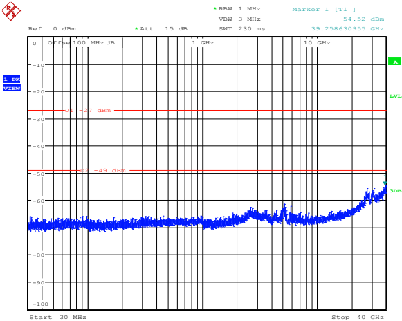
Diagram 8.5-92: Conducted spurious emissions for IC, 19 dBi antenna, 20 MHz channel, cho, high frequency
