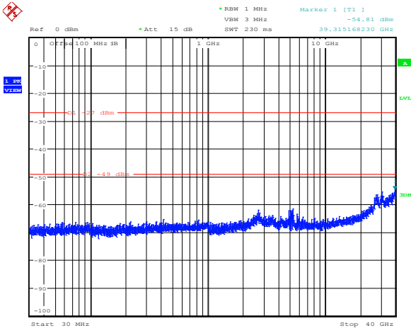
Diagram 8.5-93: Conducted spurious emissions for IC, 19 dBi antenna, 20 MHz channel, ch1, low frequency
