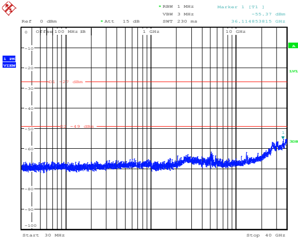
Diagram 8.5-27: Conducted spurious emissions for FCC, 19 dBi antenna, 5 MHz channel, ch1, low frequency
