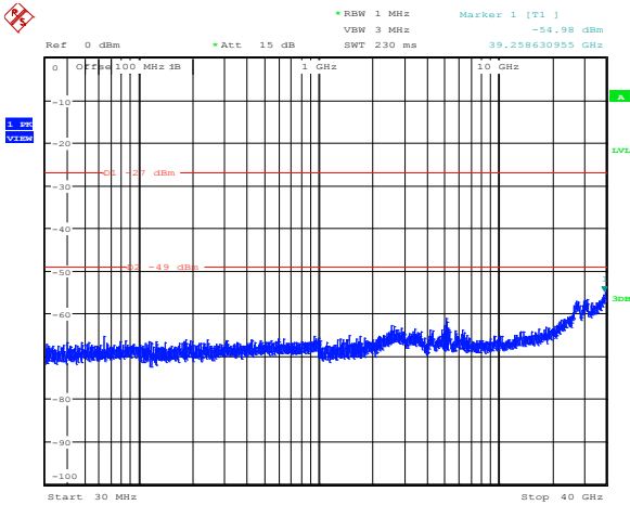
Diagram 8.5-77: Conducted spurious emissions for IC, 10 dBi antenna, 20 MHz channel, ch1, high frequency
