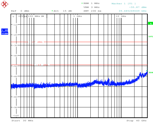
Diagram 8.5-35: Conducted spurious emissions for FCC, 19 dBi antenna, 10 MHz channel, ch1, high frequency
