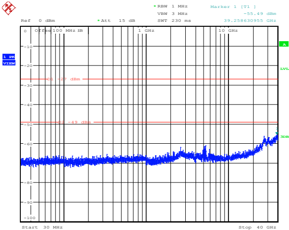
Diagram 8.5-39: Conducted spurious emissions for FCC, 19 dBi antenna, 20 MHz channel, ch1, low frequency
