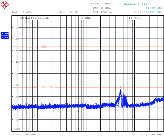
Diagram 8.5-104: Conducted spurious emissions for IC, 32 dBi antenna, 10 MHz channel, cho, high frequency
