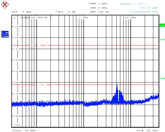
Diagram 8.5-101: Conducted spurious emissions for IC, 32 dBi antenna, 5 MHz channel, ch1, high frequency
