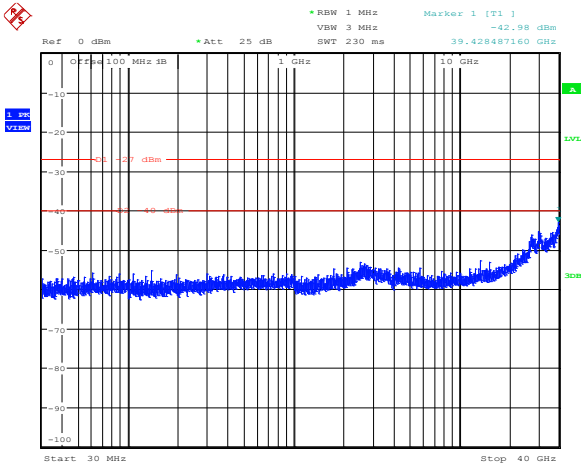
Diagram 8.5-65: Conducted spurious emissions for IC, 10 dBi antenna, 5 MHz channel, ch1, high frequency
