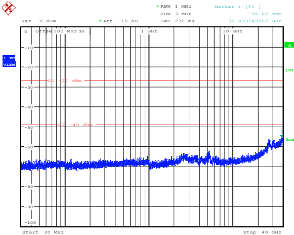
Diagram 8.5-89: Conducted spurious emissions for IC, 19 dBi antenna, 10 MHz channel, ch1, high frequency
