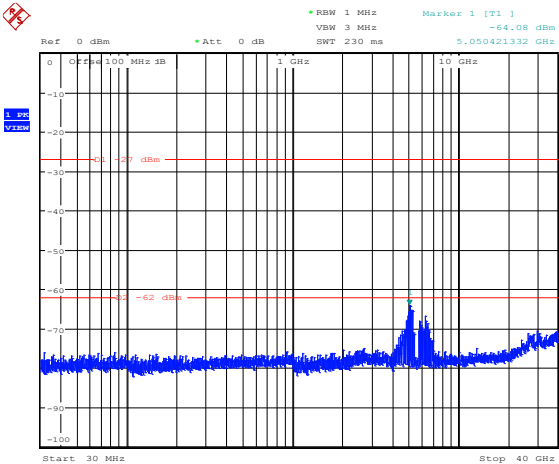
Diagram 8.5-100: Conducted spurious emissions for IC, 32 dBi antenna, 5 MHz channel, ch1, mid frequency
