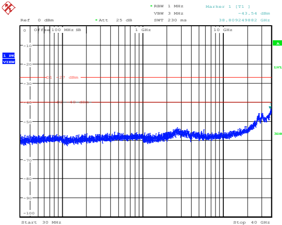
Diagram 8.5-73: Conducted spurious emissions for IC, 10 dBi antenna, 20 MHz channel, cho, mid frequency
