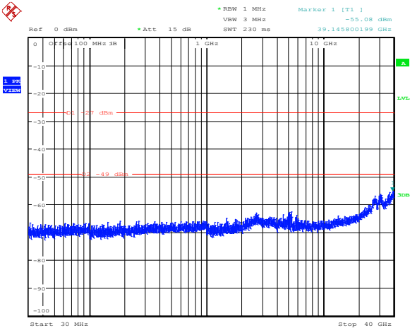
Diagram 8.5-88: Conducted spurious emissions for IC, 19 dBi antenna, 10 MHz channel, ch1, mid frequency
