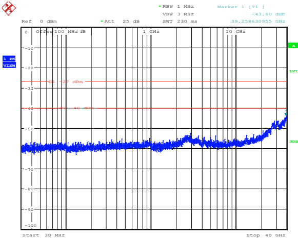
Diagram 8.5-11: Conducted spurious emissions for FCC, 10 dBi antenna, 5 MHz channel, ch1, high frequency
