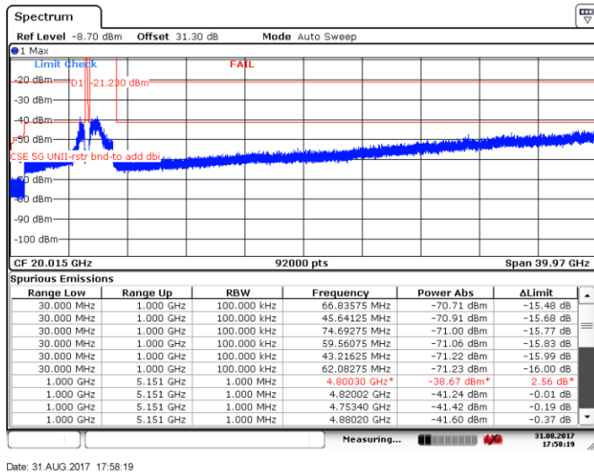
Figure 8.5-91: Spurious emissions within restricted bands, 10 MHz channel, low channel, 32 dBi antenna, cho
