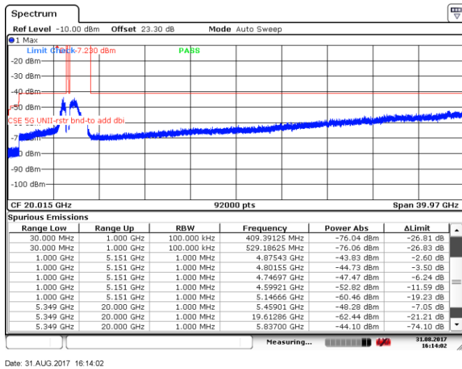
Figure 8.5-65: Spurious emissions within restricted bands, 5 MHz channel, high channel, 24 dBi antenna, cho
