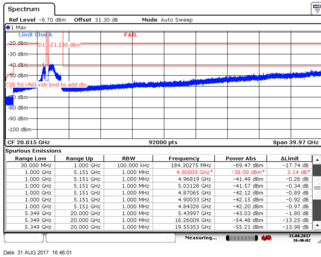
Figure 8.5-71: Spurious emissions within restricted bands, 5 MHz channel, mid channel, 32 dBi antenna, cho
