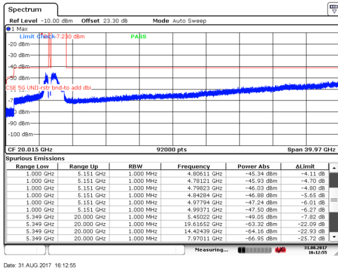
Figure 8.5-63: Spurious emissions within restricted bands, 5 MHz channel, mid channel, 24 dBi antenna, cho
