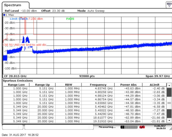
Figure 8.5-113: Spurious emissions within restricted bands, 20 MHz channel, high channel, 24 dBi antenna, cho
