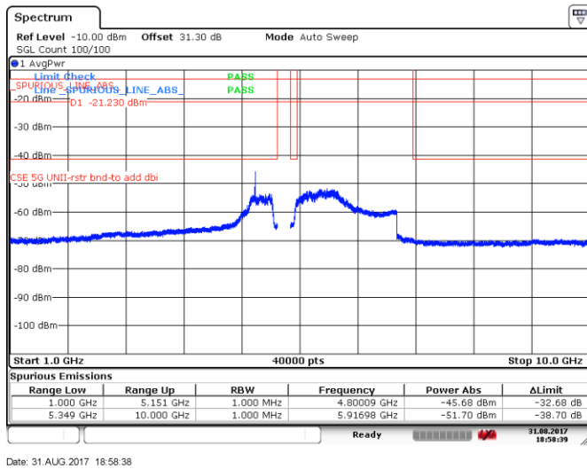
Figure 8.5-93: Spurious emissions within restricted bands (RMS zoomed), 10 MHz channel, low channel, 32 dBi antenna, cho
