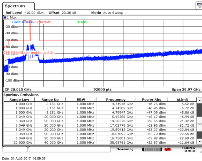
Figure 8.5-61: Spurious emissions within restricted bands, 5 MHz channel, low channel, 24 dBi antenna, cho
