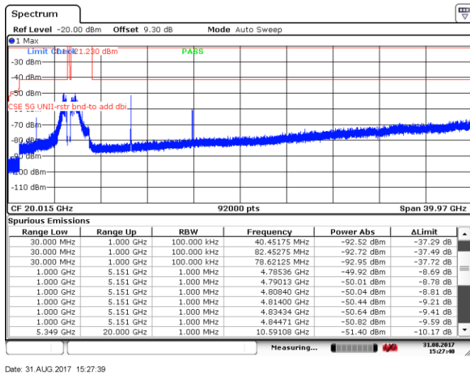
Figure 8.5-105: Spurious emissions within restricted bands, 20 MHz channel, mid channel, 10 dBi antenna, cho
