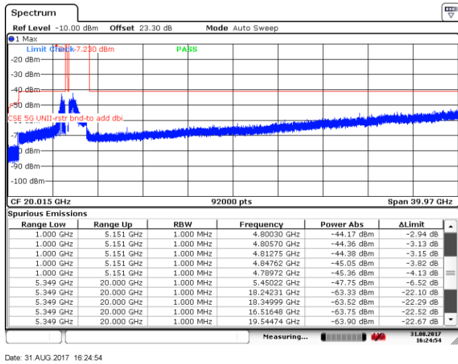
Figure 8.5-111: Spurious emissions within restricted bands, 20 MHz channel, mid channel, 24 dBi antenna, cho
