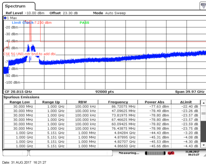
Figure 8.5-89: Spurious emissions within restricted bands, 10 MHz channel, high channel, 24 dBi antenna, cho
