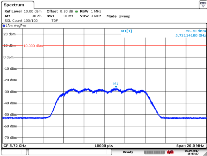
Figure 8.4-2: Sample plot for PSD on 10 MHz channel
