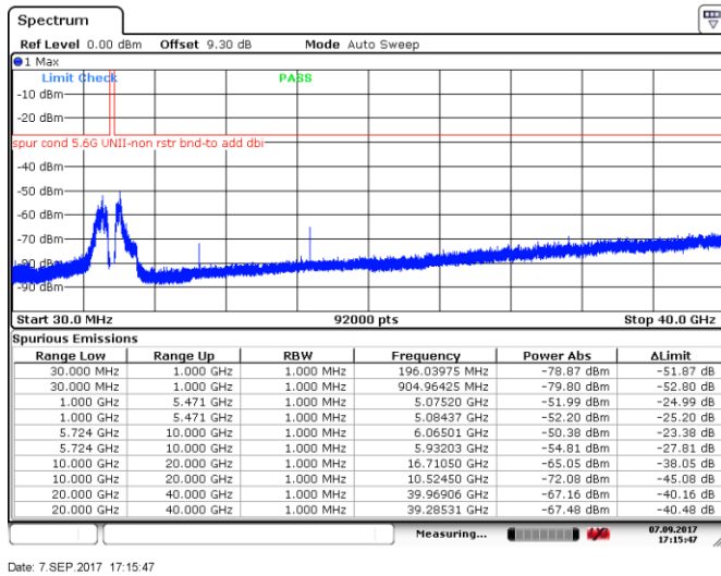
Figure 8.5-3: Spurious emissions outside restricted bands, 5 MHz channel, mid channel, 10 dBi antenna, cho
