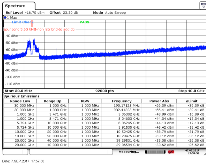
Figure 8.5-45: Spurious emissions outside restricted bands, 20 MHz channel, mid channel, 24 dBi antenna, cho
