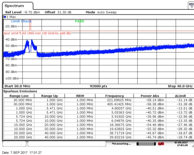
Figure 8.5-35: Spurious emissions outside restricted bands, 10 MHz channel, high channel, 32 dBi antenna, cho
