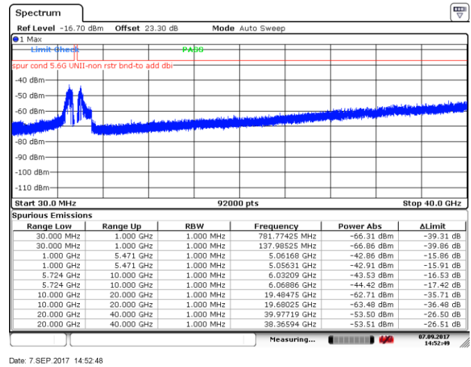
Figure 8.5-46: Spurious emissions outside restricted bands, 20 MHz channel, mid channel, 24 dBi antenna, ch1
