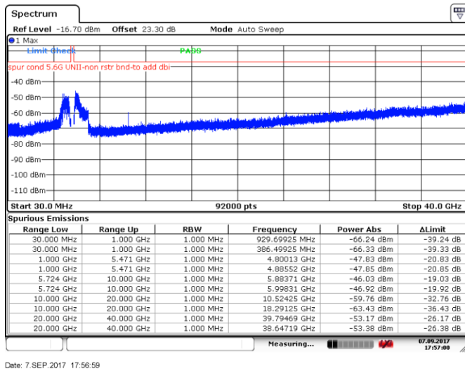
Figure 8.5-47: Spurious emissions outside restricted bands, 20 MHz channel, high channel, 24 dBi antenna, cho
