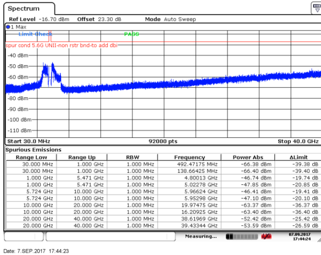
Figure 8.5-7: Spurious emissions outside restricted bands, 5 MHz channel, low channel, 24 dBi antenna, cho
