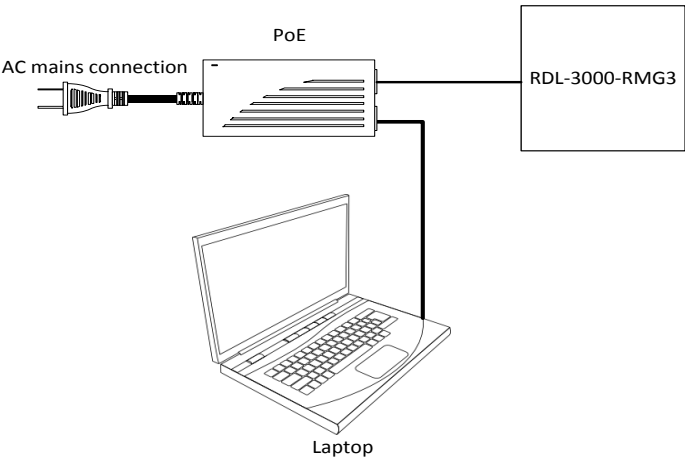
Figure 3.6-1: Setup diagram
