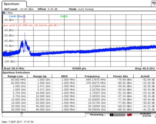
Figure 8.5-5: Spurious emissions outside restricted bands, 5 MHz channel, high channel, 10 dBi antenna, cho
