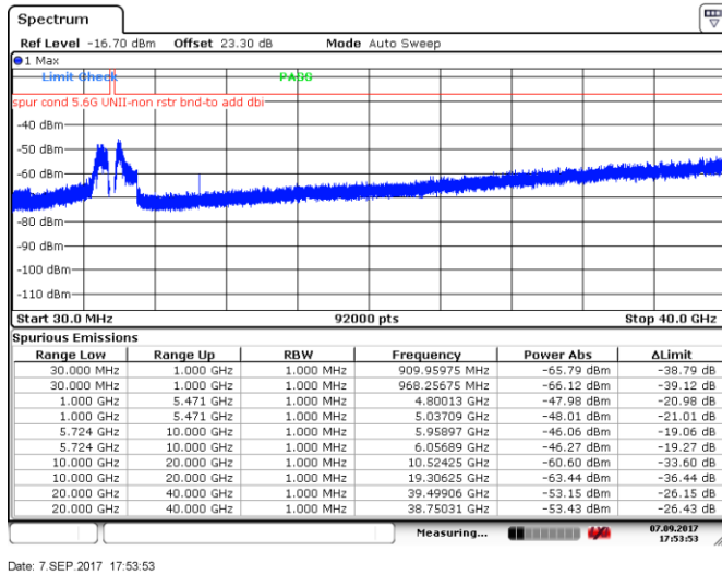
Figure 8.5-27: Spurious emissions outside restricted bands, 10 MHz channel, mid channel, 24 dBi antenna, cho
