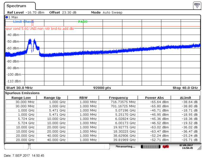
Figure 8.5-48: Spurious emissions outside restricted bands, 20 MHz channel, high channel, 24 dBi antenna, ch1
