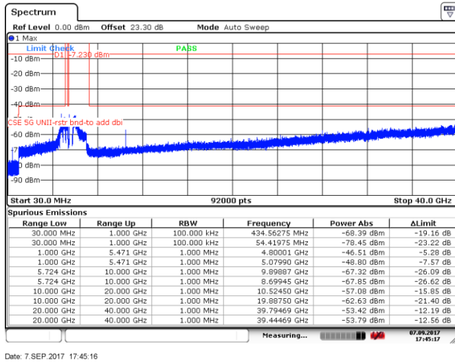
Figure 8.5-61: Spurious emissions within restricted bands, 5 MHz channel, low channel, 24 dBi antenna, cho
