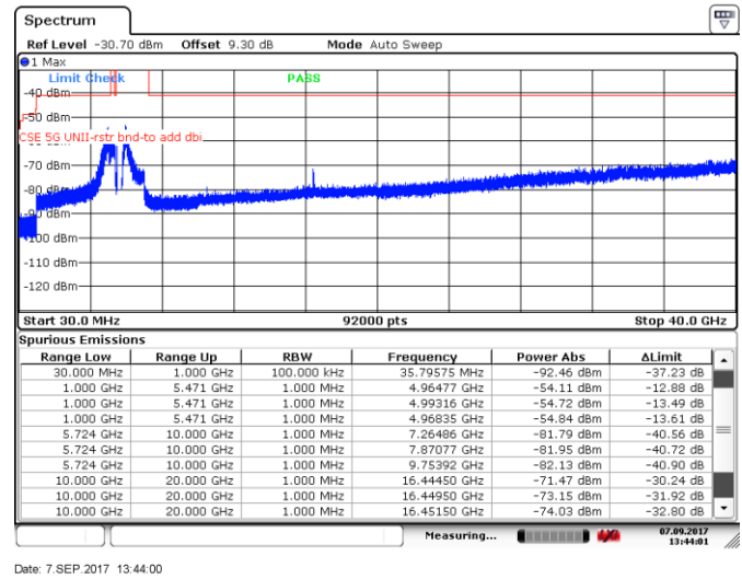
Figure 8.5-104: Spurious emissions within restricted bands, 20 MHz channel, low channel, 10 dBi antenna, ch1
