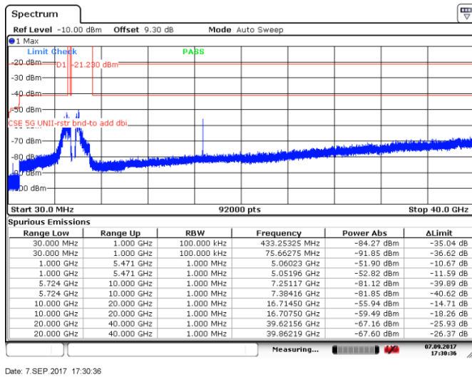
Figure 8.5-81: Spurious emissions within restricted bands, 10 MHz channel, mid channel, 10 dBi antenna, cho
