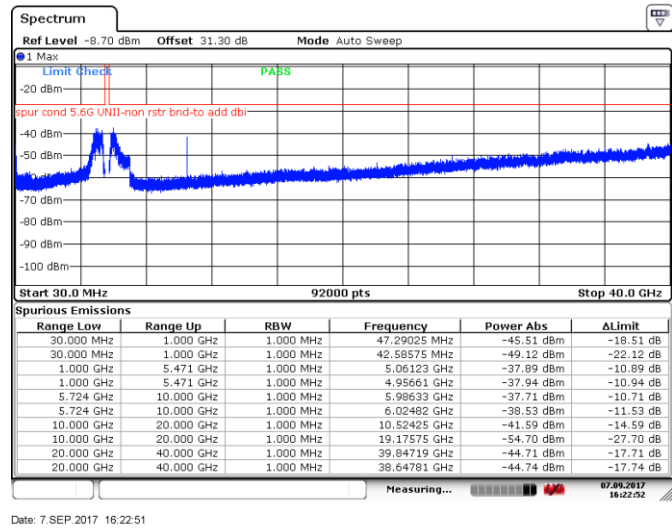
Figure 8.5-50: Spurious emissions outside restricted bands, 20 MHz channel, low channel, 32 dBi antenna, ch1
