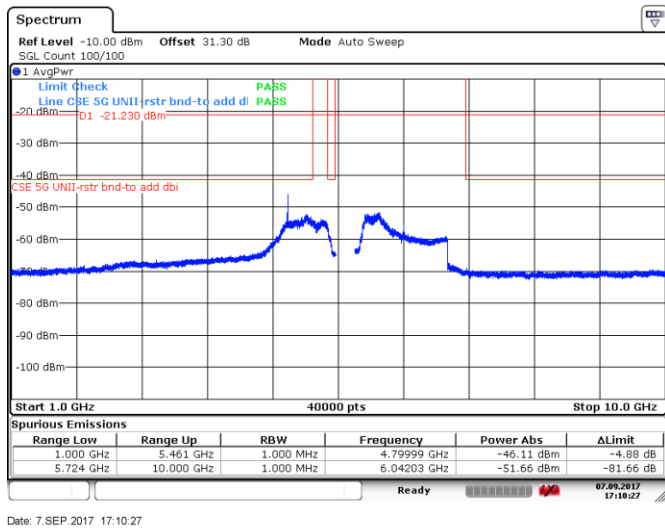
Figure 8.5-73: Spurious emissions within restricted bands (RMS zoomed), 5 MHz channel, mid channel, 32 dBi antenna, cho
