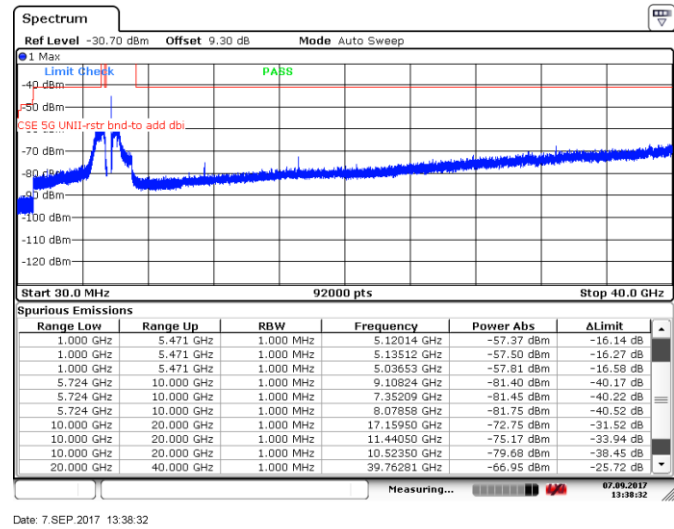
Figure 8.5-84: Spurious emissions within restricted bands, 10 MHz channel, high channel, 10 dBi antenna, ch1
