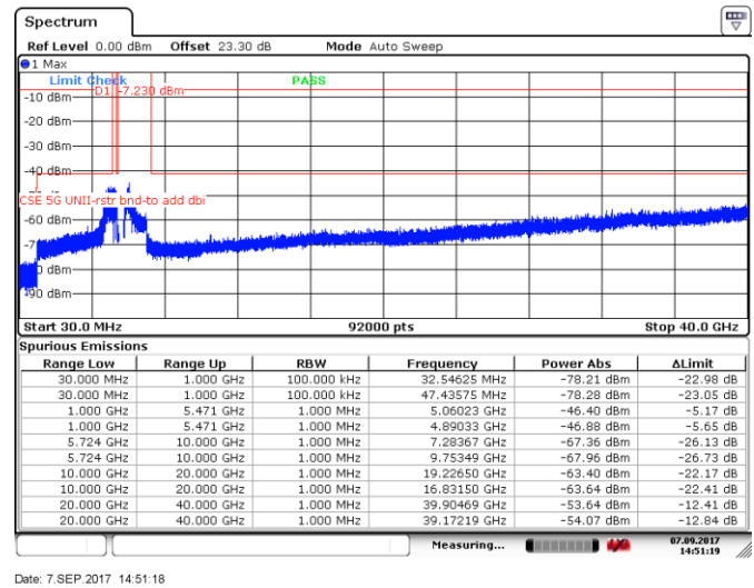
Figure 8.5-114: Spurious emissions within restricted bands, 20 MHz channel, high channel, 24 dBi antenna, ch1
