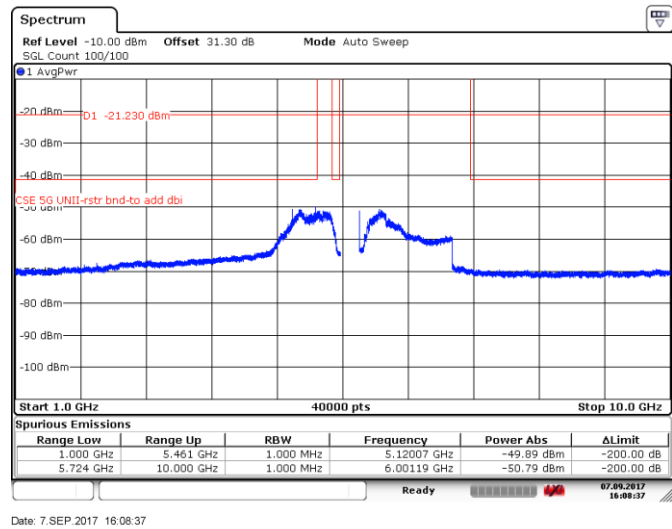
Figure 8.5-78: Spurious emissions within restricted bands (RMS zoomed), 5 MHz channel, high channel, 32 dBi antenna, ch1
