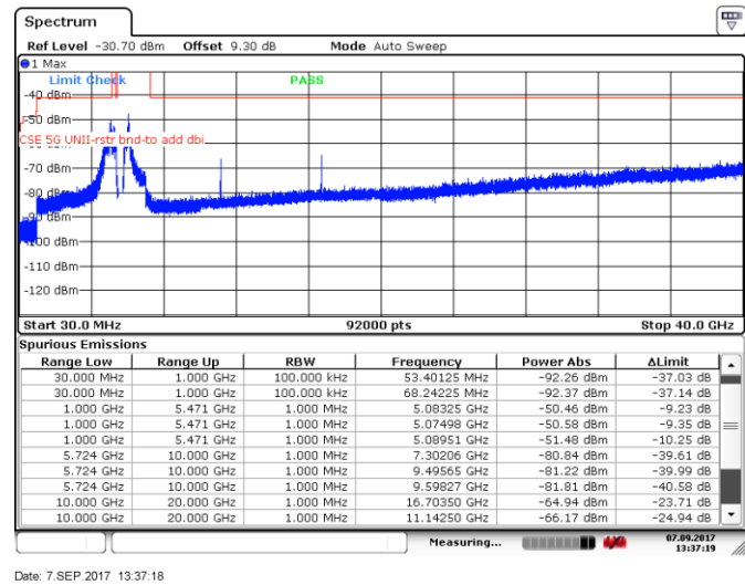
Figure 8.5-82: Spurious emissions within restricted bands, 10 MHz channel, mid channel, 10 dBi antenna, ch1
