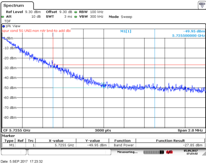
Figure 8.5-129: Upper band edge for FCC, 5 MHz channel, 10 dBi antenna, ch0
