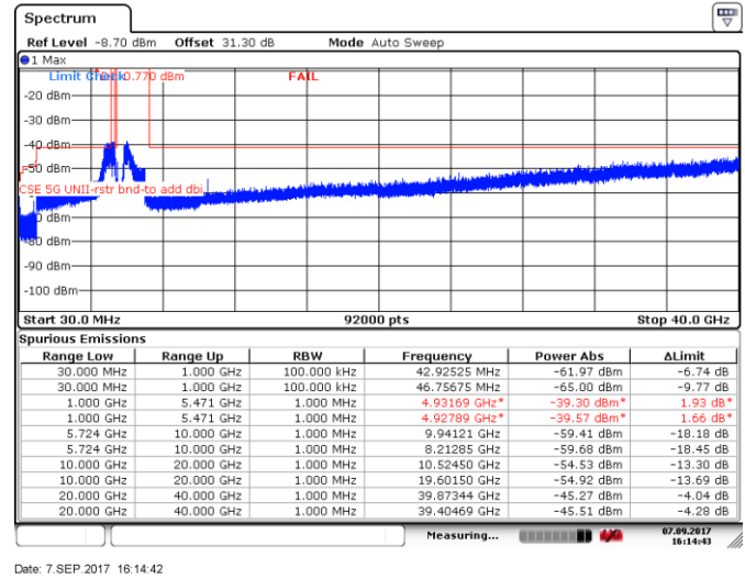
Figure 8.5-92: Spurious emissions within restricted bands, 10 MHz channel, low channel, 32 dBi antenna, ch1
