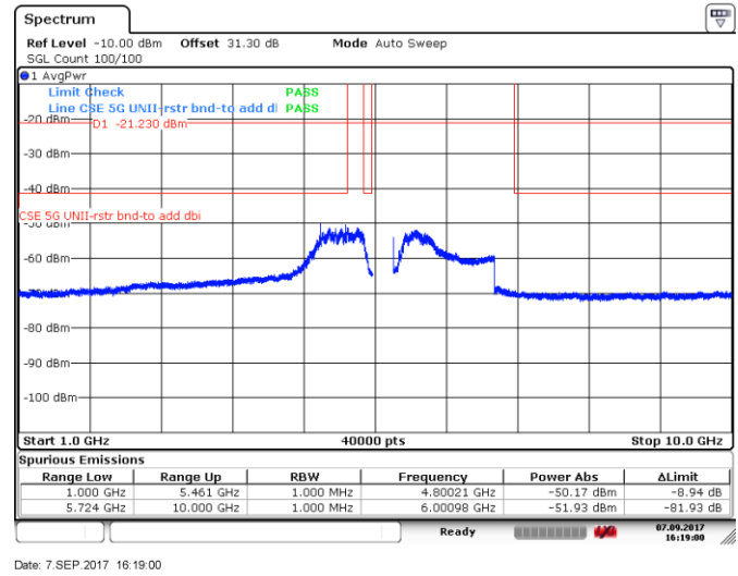
Figure 8.5-102: Spurious emissions within restricted bands (RMS zoomed), 10 MHz channel, high channel, 32 dBi antenna, ch1
