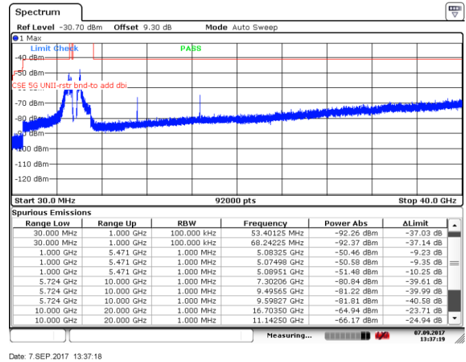
Figure 8.5-106: Spurious emissions within restricted bands, 20 MHz channel, mid channel, 10 dBi antenna, ch1
