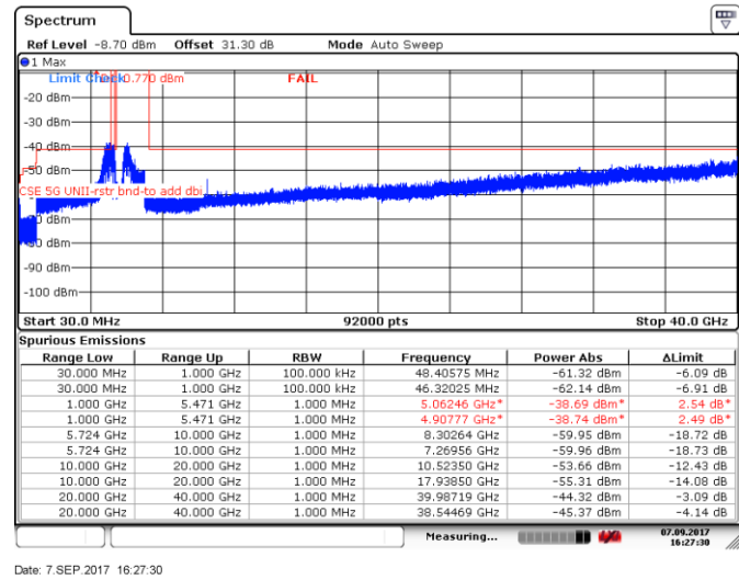
Figure 8.5-120: Spurious emissions within restricted bands, 20 MHz channel, mid channel, 32 dBi antenna, ch1
