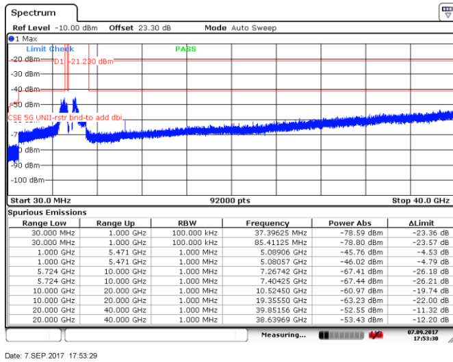
Figure 8.5-87: Spurious emissions within restricted bands, 10 MHz channel, mid channel, 24 dBi antenna, cho
