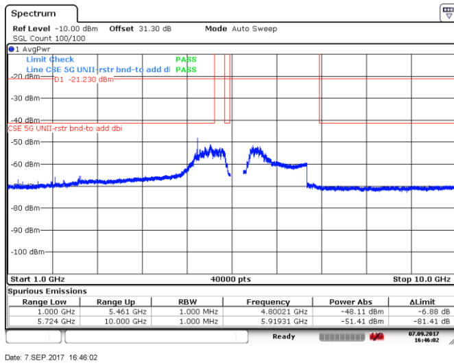
Figure 8.5-121: Spurious emissions within restricted bands (RMS zoomed), 20 MHz channel, mid channel, 32 dBi antenna, cho
