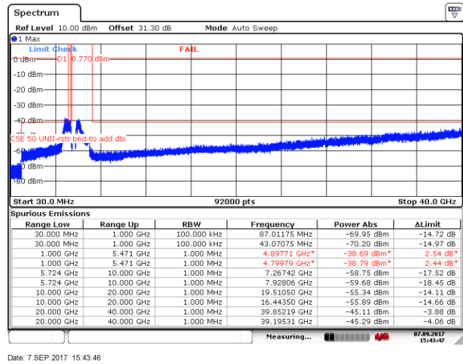
Figure 8.5-72: Spurious emissions within restricted bands, 5 MHz channel, mid channel, 32 dBi antenna, ch1
