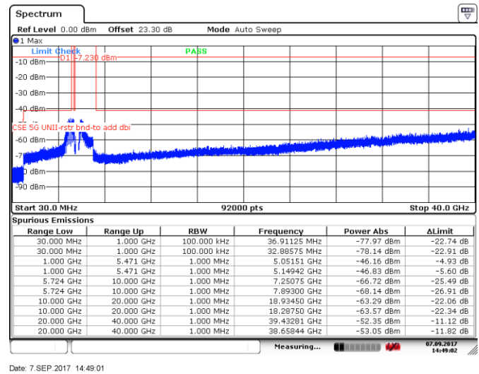
Figure 8.5-110: Spurious emissions within restricted bands, 20MHz channel, low channel, 24 dBi antenna, ch1
