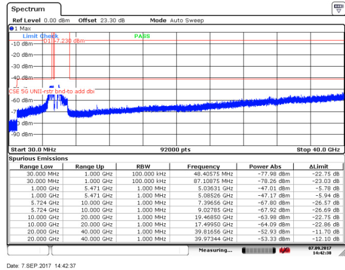
Figure 8.5-86: Spurious emissions within restricted bands, 10 MHz channel, low channel, 24 dBi antenna, ch1
