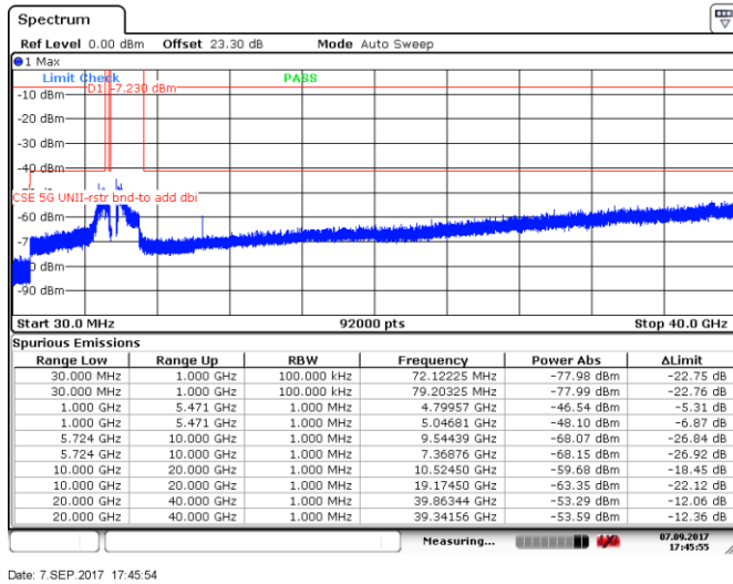
Figure 8.5-65: Spurious emissions within restricted bands, 5 MHz channel, high channel, 24 dBi antenna, cho
