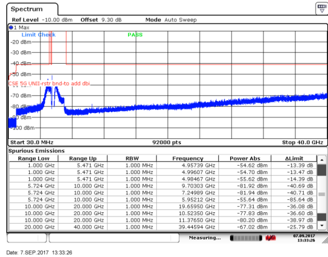
Figure 8.5-80: Spurious emissions within restricted bands, 10 MHz channel, low channel, 10 dBi antenna, ch1
