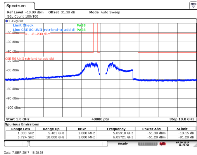
Figure 8.5-122: Spurious emissions within restricted bands (RMS zoomed), 20 MHz channel, mid channel, 32 dBi antenna, ch1
