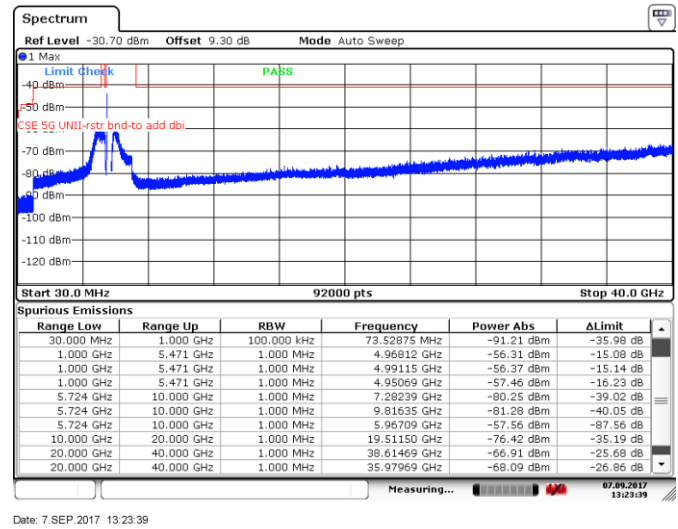
Figure 8.5-56: Spurious emissions within restricted bands, 5 MHz channel, low channel, 10 dBi antenna, ch1
