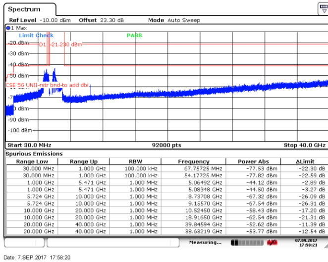
Figure 8.5-111: Spurious emissions within restricted bands, 20 MHz channel, mid channel, 24 dBi antenna, cho
