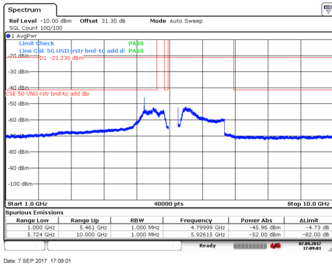
Figure 8.5-77: Spurious emissions within restricted bands (RMS zoomed), 5 MHz channel, high channel, 32 dBi antenna, cho
