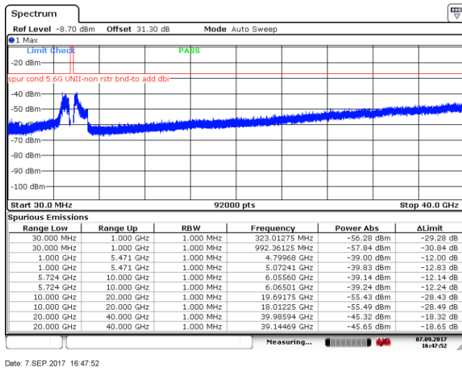
Figure 8.5-51: Spurious emissions outside restricted bands, 20 MHz channel, mid channel, 32 dBi antenna, cho
