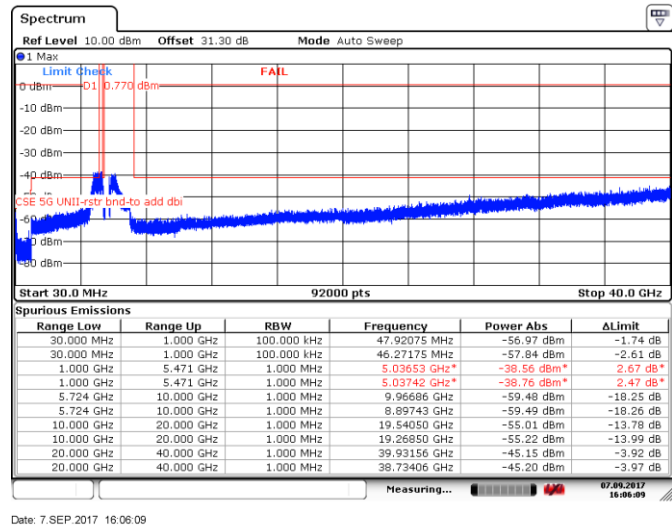
Figure 8.5-76: Spurious emissions within restricted bands, 5 MHz channel, high channel, 32 dBi antenna, ch1
