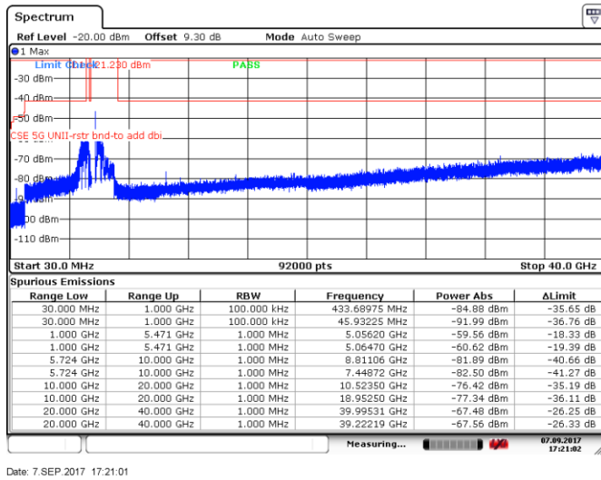
Figure 8.5-59: Spurious emissions within restricted bands, 5 MHz channel, high channel, 10 dBi antenna, cho
