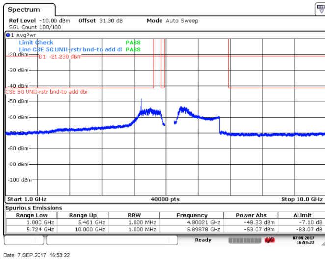
Figure 8.5-125: Spurious emissions within restricted bands (RMS zoomed), 20 MHz channel, high channel, 32 dBi antenna, cho
