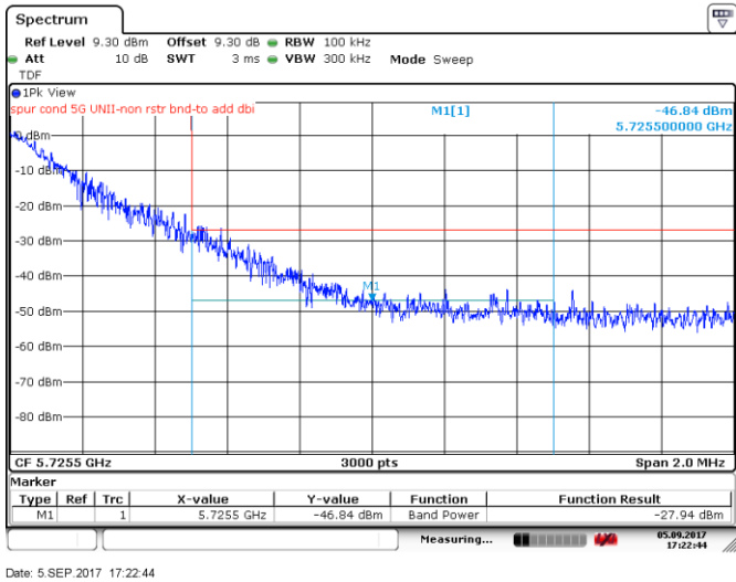
Figure 8.5-130: Upper band edge for FCC, 5 MHz channel, 10 dBi antenna, ch1
