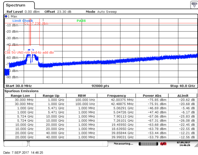
Figure 8.5-90: Spurious emissions within restricted bands, 10 MHz channel, high channel, 24 dBi antenna, ch1
