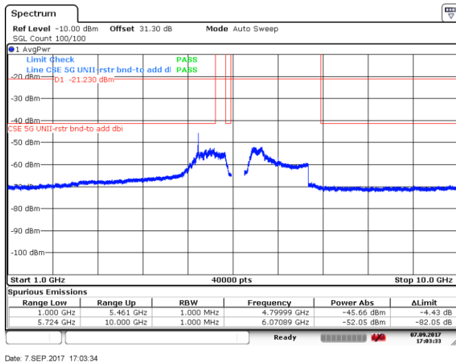
Figure 8.5-97: Spurious emissions within restricted bands (RMS zoomed), 10 MHz channel, mid channel, 32 dBi antenna, cho
