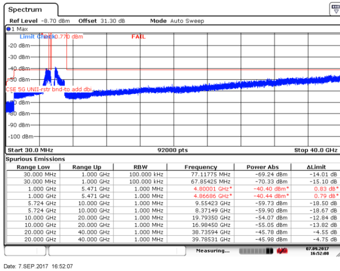
Figure 8.5-123: Spurious emissions within restricted bands, 20 MHz channel, high channel, 32 dBi antenna, cho
