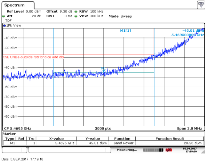
Figure 8.5-128: Lower band edge for FCC, 5 MHz channel, 10 dBi antenna, ch1
