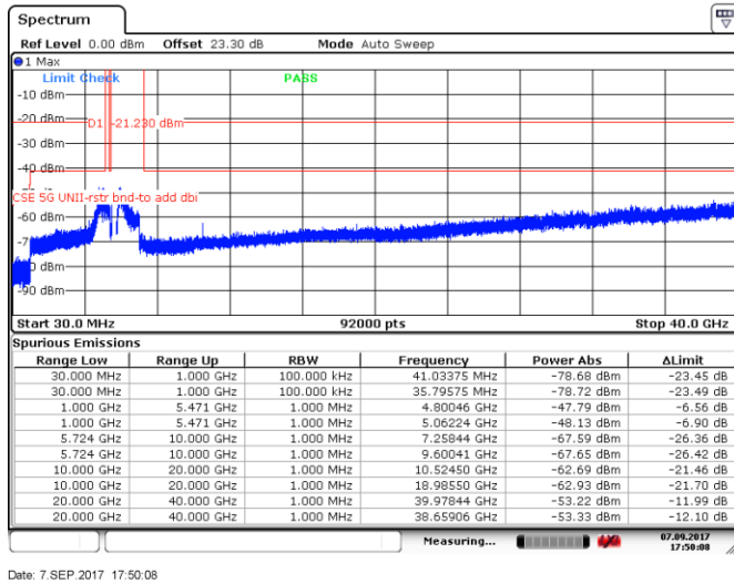
Figure 8.5-85: Spurious emissions within restricted bands, 10 MHz channel, low channel, 24 dBi antenna, cho
