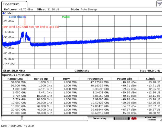
Figure 8.5-54: Spurious emissions outside restricted bands, 20 MHz channel, high channel, 32 dBi antenna, ch1
