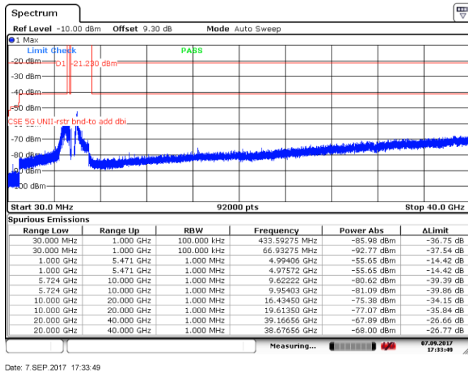
Figure 8.5-103: Spurious emissions within restricted bands, 20 MHz channel, low channel, 10 dBi antenna, cho
