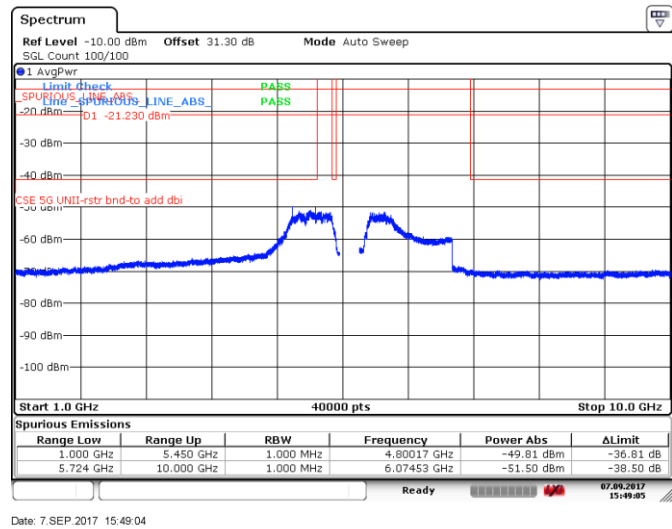
Figure 8.5-74: Spurious emissions within restricted bands (RMS zoomed), 5 MHz channel, mid channel, 32 dBi antenna, ch1
