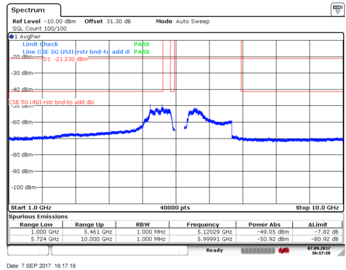
Figure 8.5-98: Spurious emissions within restricted bands (RMS zoomed), 10 MHz channel, mid channel, 32 dBi antenna, ch1
