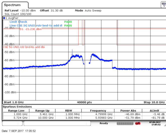
Figure 8.5-69: Spurious emissions within restricted bands (RMS zoomed), 5 MHz channel, low channel, 32 dBi antenna, cho
