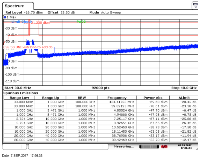
Figure 8.5-113: Spurious emissions within restricted bands, 20 MHz channel, high channel, 24 dBi antenna, cho
