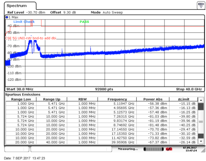
Figure 8.5-108: Spurious emissions within restricted bands, 20MHz channel, high channel, 10 dBi antenna, ch1
