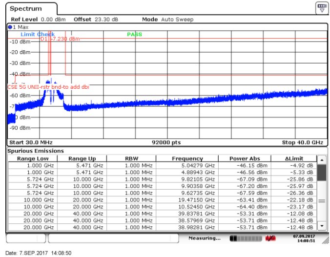
Figure 8.5-62: Spurious emissions within restricted bands, 5 MHz channel, low channel, 24 dBi antenna, ch1
