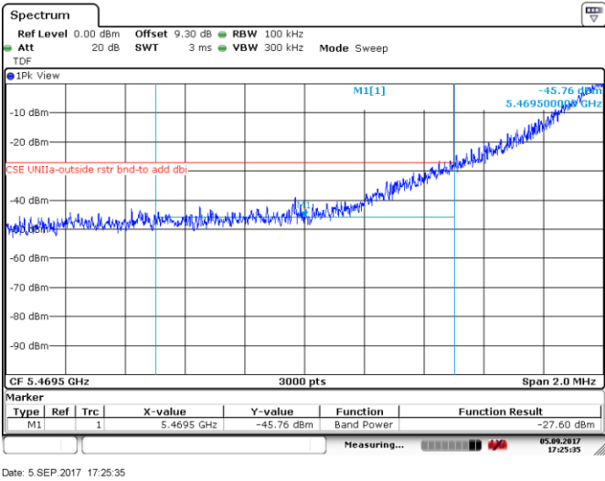
Figure 8.5-127: Lower band edge for FCC, 5 MHz channel, 10 dBi antenna, ch0
