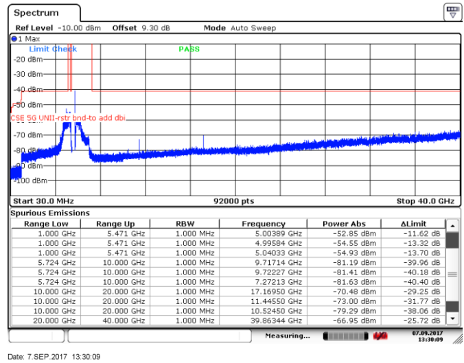
Figure 8.5-60: Spurious emissions within restricted bands, 5 MHz channel, high channel, 10 dBi antenna, ch1
