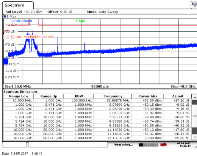
Figure 8.5-105: Spurious emissions within restricted bands, 20 MHz channel, mid channel, 10 dBi antenna, cho
