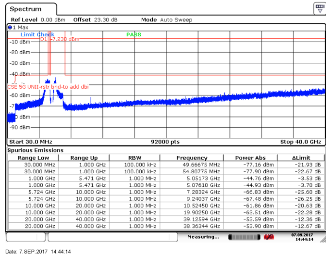
Figure 8.5-88: Spurious emissions within restricted bands, 10 MHz channel, mid channel, 24 dBi antenna, ch1
