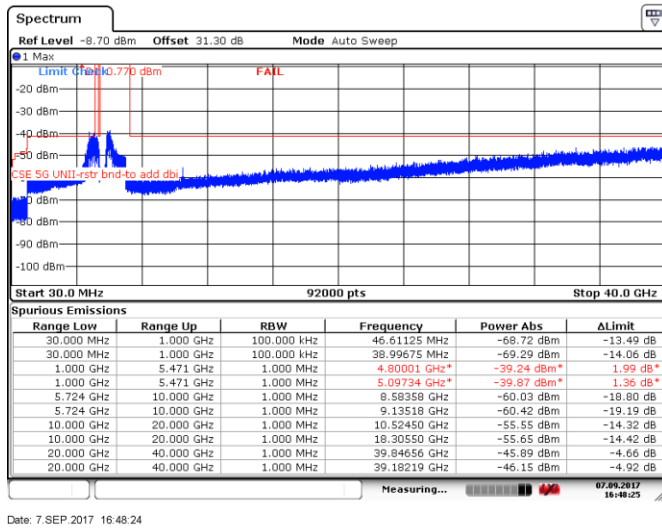
Figure 8.5-119: Spurious emissions within restricted bands, 20 MHz channel, mid channel, 32 dBi antenna, cho
