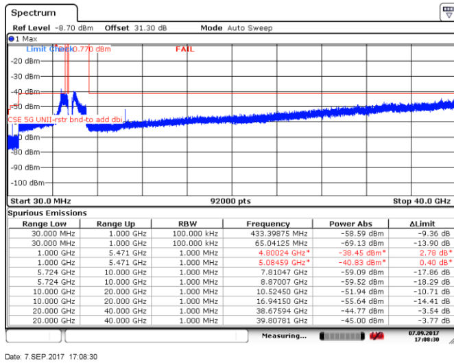
Figure 8.5-75: Spurious emissions within restricted bands, 5 MHz channel, high channel, 32 dBi antenna, cho
