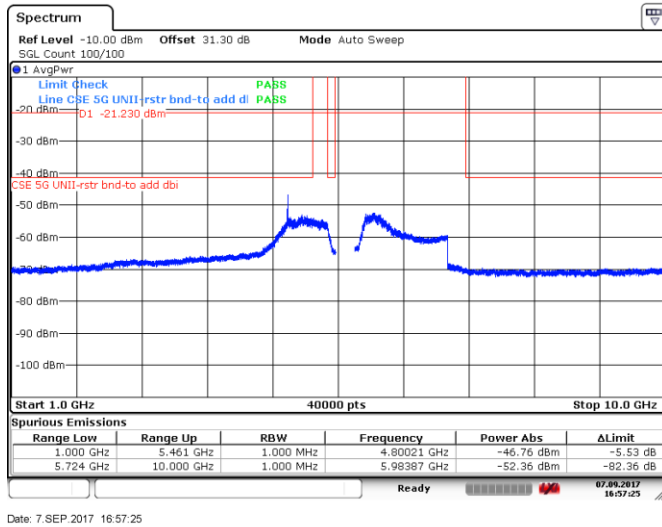
Figure 8.5-93: Spurious emissions within restricted bands (RMS zoomed), 10 MHz channel, low channel, 32 dBi antenna, cho
