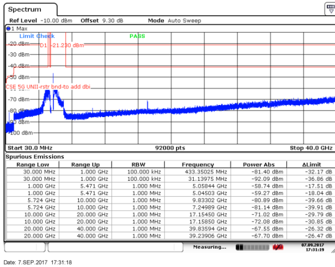
Figure 8.5-83: Spurious emissions within restricted bands, 10 MHz channel, high channel, 10 dBi antenna, cho
