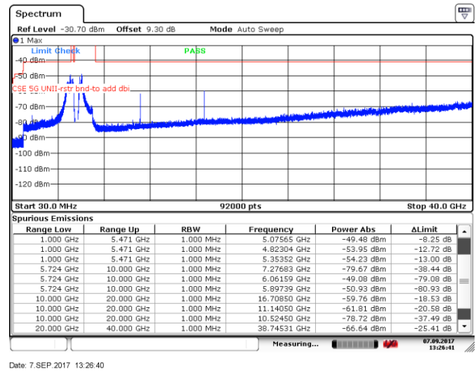
Figure 8.5-58: Spurious emissions within restricted bands, 5 MHz channel, mid channel, 10 dBi antenna, ch1
