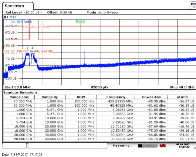
Figure 8.5-57: Spurious emissions within restricted bands, 5 MHz channel, mid channel, 10 dBi antenna, cho
