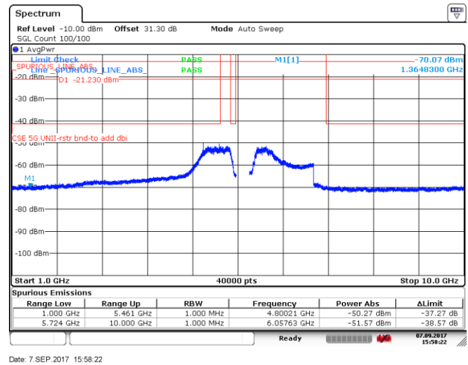
Figure 8.5-70: Spurious emissions within restricted bands (RMS zoomed), 5 MHz channel, low channel, 32 dBi antenna, ch1
