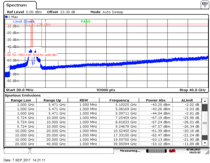
Figure 8.5-64: Spurious emissions within restricted bands, 5 MHz channel, mid channel, 24 dBi antenna, ch1
