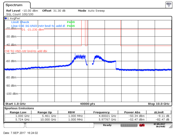
Figure 8.5-118: Spurious emissions within restricted bands (RMS zoomed), 20 MHz channel, low channel, 32 dBi antenna, ch1
