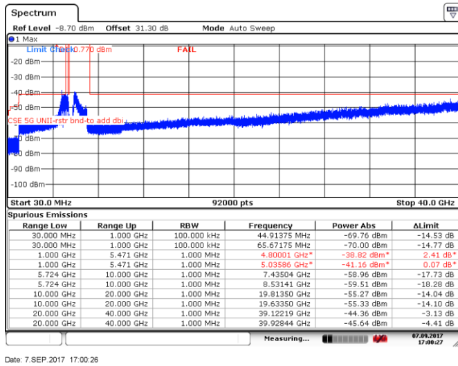
Figure 8.5-99: Spurious emissions within restricted bands, 10 MHz channel, high channel, 32 dBi antenna, cho
