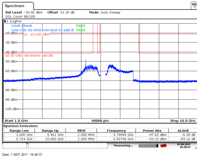
Figure 8.5-117: Spurious emissions within restricted bands (RMS zoomed), 20 MHz channel, low channel, 32 dBi antenna, cho
