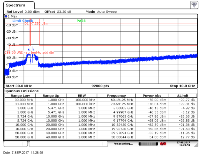
Figure 8.5-66: Spurious emissions within restricted bands, 5 MHz channel, high channel, 24 dBi antenna, ch1
