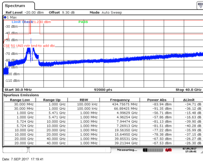
Figure 8.5-55: Spurious emissions within restricted bands, 5 MHz channel, low channel, 10 dBi antenna, cho
