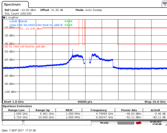
Figure 8.5-101: Spurious emissions within restricted bands (RMS zoomed), 10 MHz channel, high channel, 32 dBi antenna, cho
