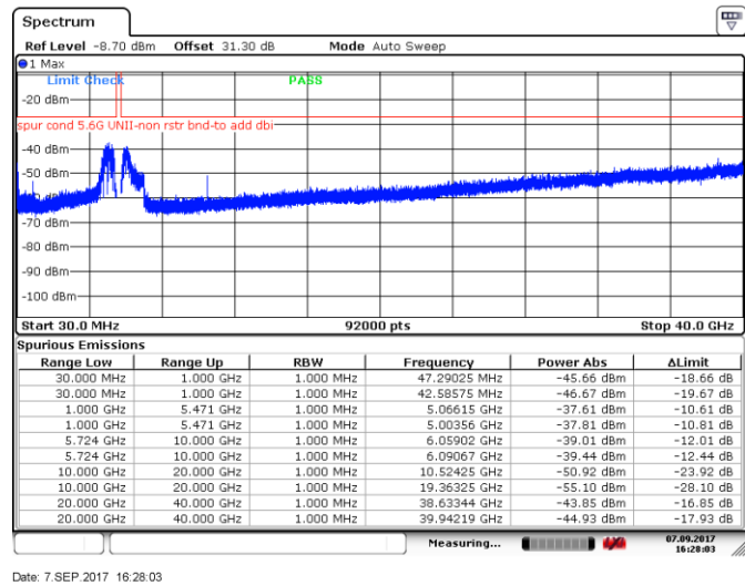
Figure 8.5-52: Spurious emissions outside restricted bands, 20 MHz channel, mid channel, 32 dBi antenna, ch1
