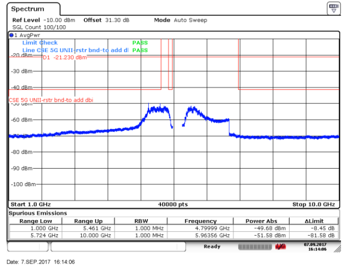
Figure 8.5-94: Spurious emissions within restricted bands (RMS zoomed), 10 MHz channel, low channel, 32 dBi antenna, ch1
