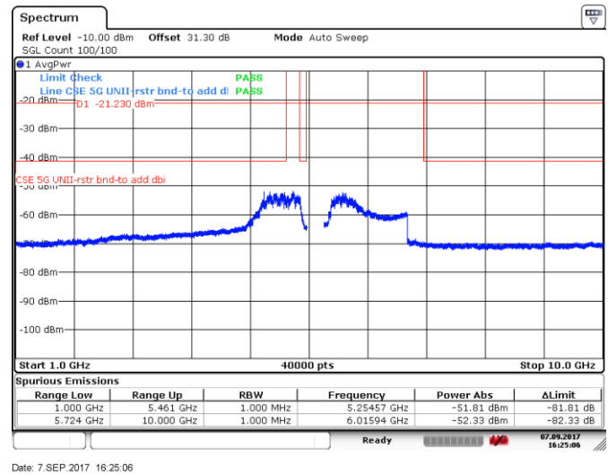
Figure 8.5-126: Spurious emissions within restricted bands (RMS zoomed), 20 MHz channel, high channel, 32 dBi antenna, ch1
