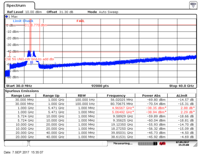
Figure 8.5-68: Spurious emissions within restricted bands, 5 MHz channel, low channel, 32 dBi antenna, ch1
