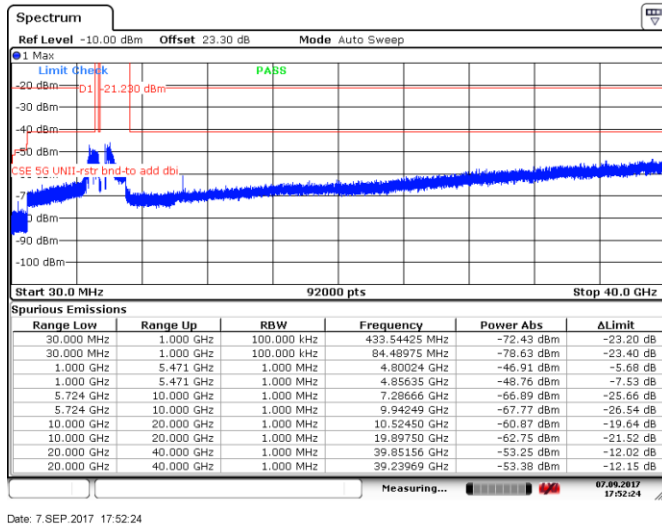
Figure 8.5-89: Spurious emissions within restricted bands, 10 MHz channel, high channel, 24 dBi antenna, cho
