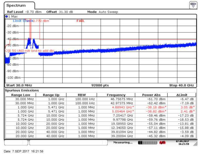
Figure 8.5-116: Spurious emissions within restricted bands, 20 MHz channel, low channel, 32 dBi antenna, ch1
