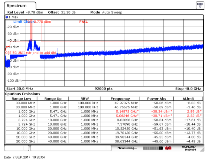
Figure 8.5-124: Spurious emissions within restricted bands, 20 MHz channel, high channel, 32 dBi antenna, ch1
