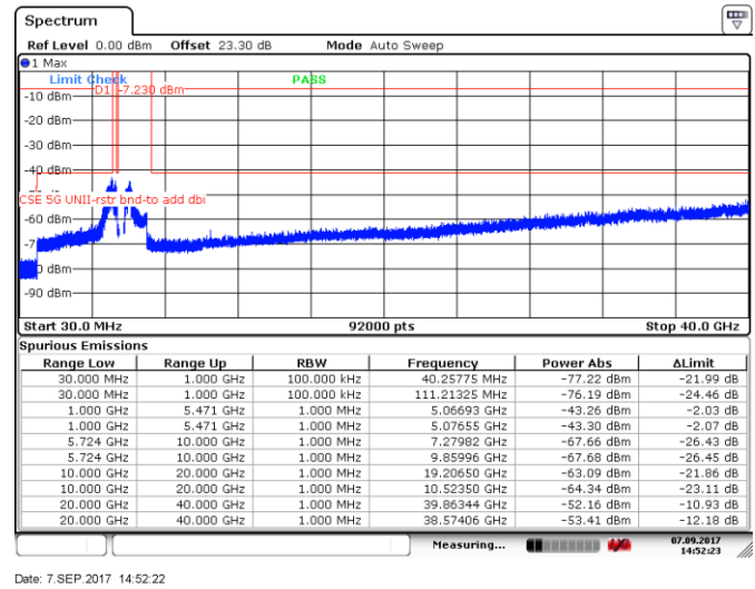
Figure 8.5-112: Spurious emissions within restricted bands, 20 MHz channel, mid channel, 24 dBi antenna, ch1
