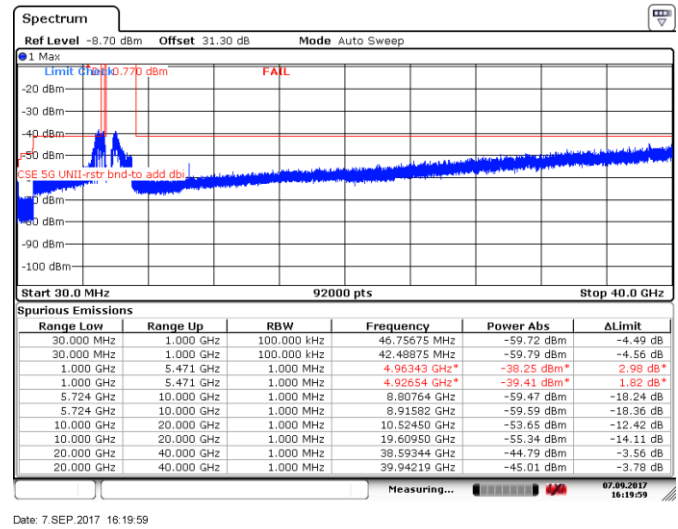
Figure 8.5-100: Spurious emissions within restricted bands, 10 MHz channel, high channel, 32 dBi antenna, ch1
