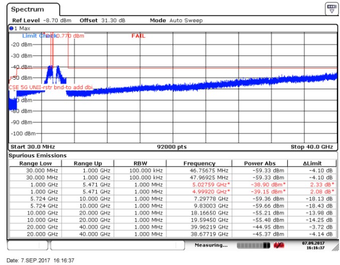
Figure 8.5-96: Spurious emissions within restricted bands, 10 MHz channel, mid channel, 32 dBi antenna, ch1
