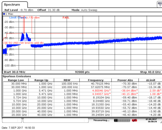
Figure 8.5-115: Spurious emissions within restricted bands, 20 MHz channel, low channel, 32 dBi antenna, cho
