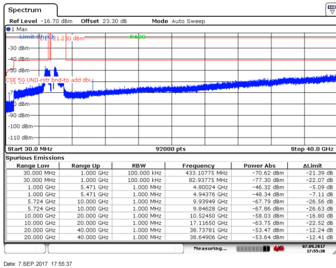
Figure 8.5-109: Spurious emissions within restricted bands, 20 MHz channel, low channel, 24 dBi antenna, cho
