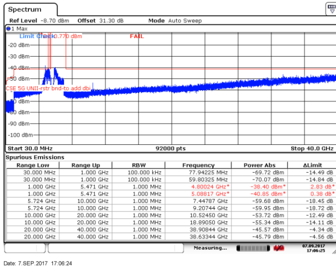
Figure 8.5-67: Spurious emissions within restricted bands, 5 MHz channel, low channel, 32 dBi antenna, cho
