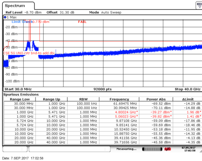
Figure 8.5-95: Spurious emissions within restricted bands, 10 MHz channel, mid channel, 32 dBi antenna, cho
