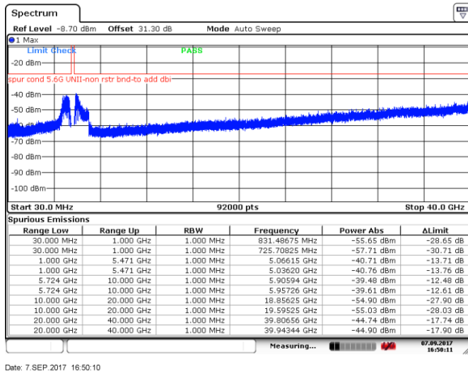
Figure 8.5-49: Spurious emissions outside restricted bands, 20 MHz channel, low channel, 32 dBi antenna, cho
