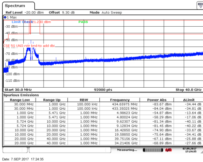
Figure 8.5-79: Spurious emissions within restricted bands, 10 MHz channel, low channel, 10 dBi antenna, cho
