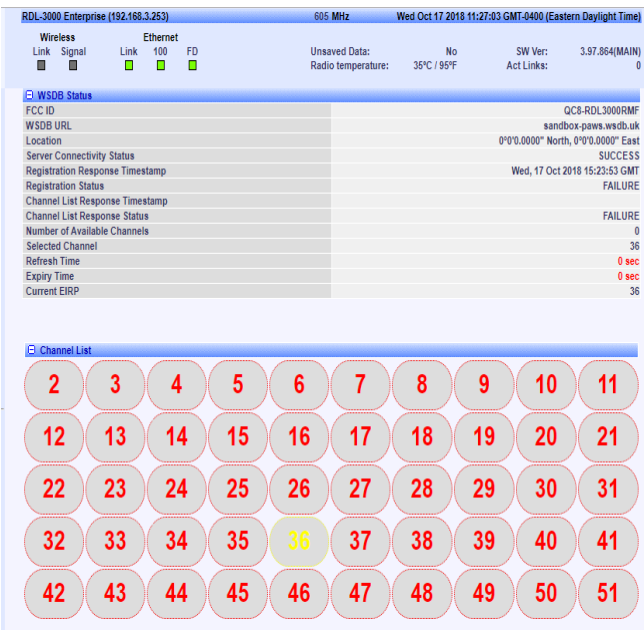
Figure 8.3-4: Data log of unsuccessful registration with restricted coordinates of Subscriber device and reception of empty channel list
