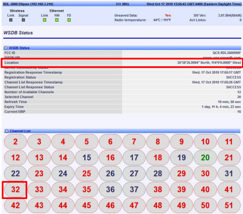
Figure 8.19-3: Received channel list for coordinates set in scenarios (a) and (b). DTS channel 32 at location coordinates 35.66N, 114.0W
