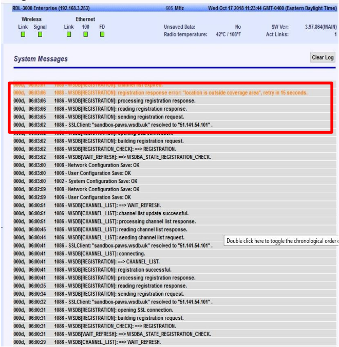
Figure 8.3-4: Data log of unsuccessful registration with restricted coordinates of Subscriber device and reception of empty channel list
