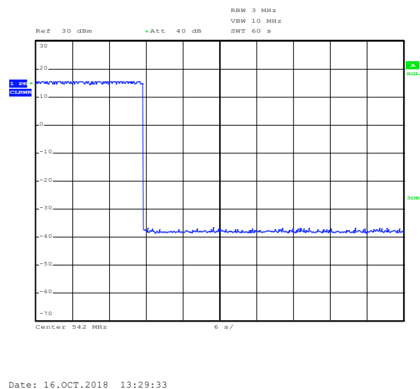
Figure 8.3-1: Unsuccessful registration with restricted coordinates. Spectrum plot shows that prior to the unsuccessful registration the EUT was transmitting and the transmission stopped right after the EUT detected missing information in the registration form.
