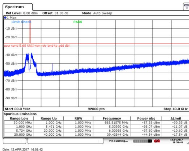
Figure 8.4-191: Spurious emissions outside restricted bands, 20 MHz channel, high channel, 32 dBi antenna, cho, 256-QAM
