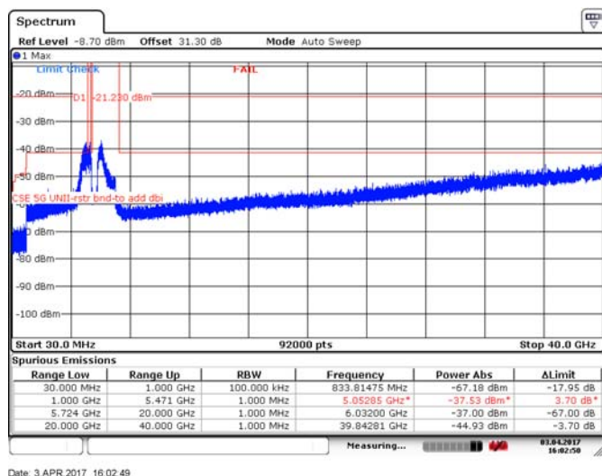
Figure 8.4-215: Spurious emissions within restricted bands, 10 MHz channel, mid channel, 32 dBi antenna, cho, 256-QAM
