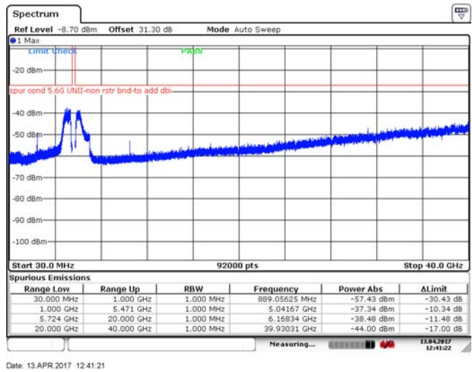
Figure 8.4-184: Spurious emissions outside restricted bands, 20 MHz channel, low channel, 32 dBi antenna, ch1, 256QAM
