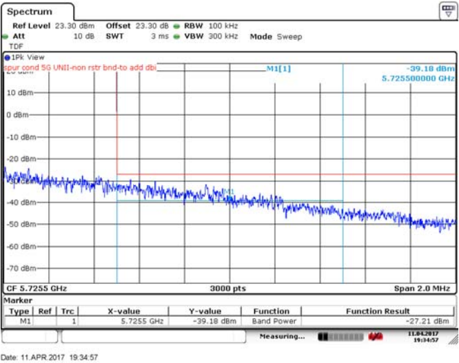
Figure 8.4-162: Upper band edge for FCC, 20 MHz channel, 24 dBi antenna, BPSK
