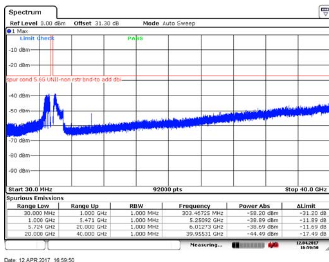
Figure 8.4-189: Spurious emissions outside restricted bands, 20 MHz channel, high channel, 32 dBi antenna, cho, BPSK
