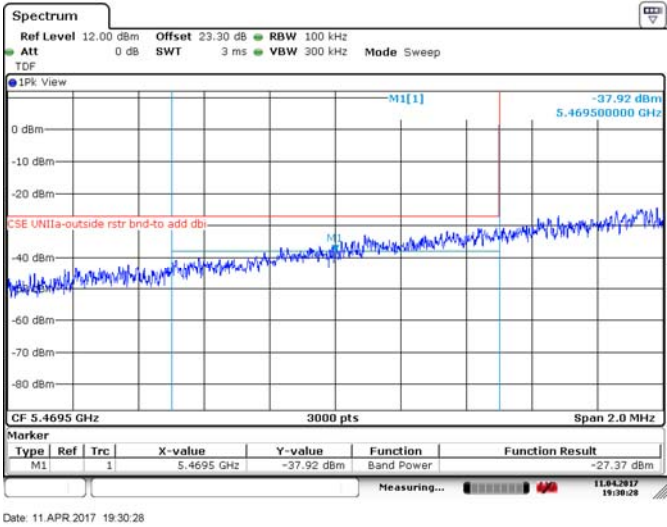
Figure 8.4-163: Lower band edge for FCC, 20 MHz channel, 24 dBi antenna, 256QAM
