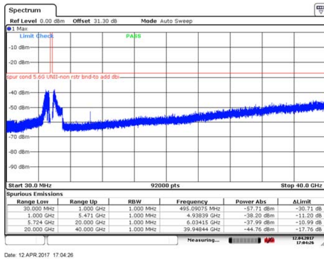
Figure 8.4-193: Spurious emissions outside restricted bands, 40 MHz channel, low channel, 32 dBi antenna, cho, BPSK
