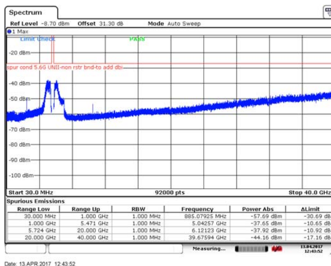
Figure 8.4-186: Spurious emissions outside restricted bands, 20 MHz channel, mid channel, 32 dBi antenna, ch1, BPSK
