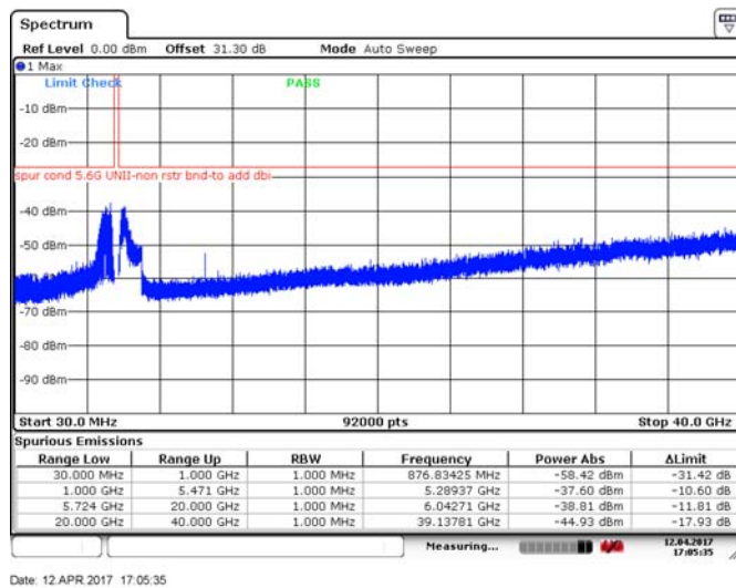
Figure 8.4-195: Spurious emissions outside restricted bands, 40 MHz channel, low channel, 32 dBi antenna, cho, 256QAM
