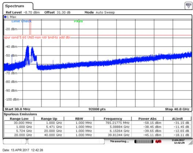
Figure 8.4-182: Spurious emissions outside restricted bands, 20 MHz channel, low channel, 32 dBi antenna, ch1, BPSK
