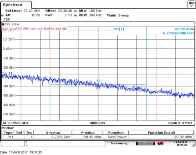
Figure 8.4-164: Upper band edge for FCC, 20 MHz channel, 24 dBi antenna, 256QAM
