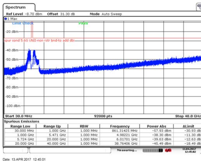
Figure 8.4-188: Spurious emissions outside restricted bands, 20 MHz channel, mid channel, 32 dBi antenna, ch1, 256-QAM
