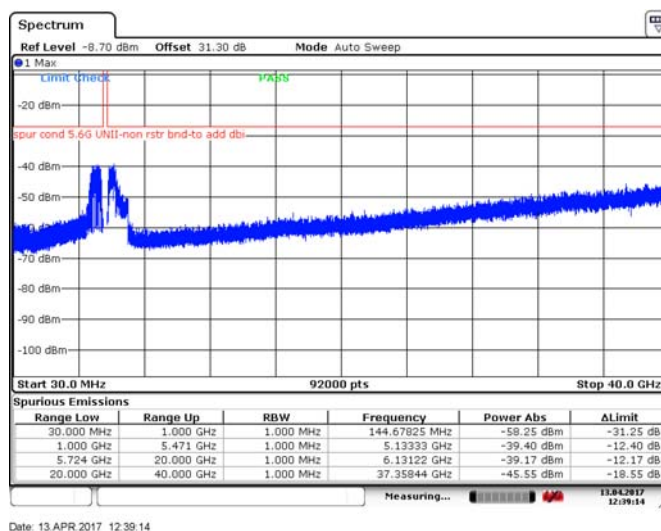
Figure 8.4-190: Spurious emissions outside restricted bands, 20 MHz channel, high channel, 32 dBi antenna, ch1, BPSK
