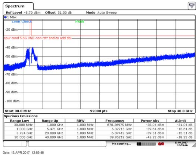
Figure 8.4-194: Spurious emissions outside restricted bands, 40 MHz channel, low channel, 32 dBi antenna, ch1, BPSK
