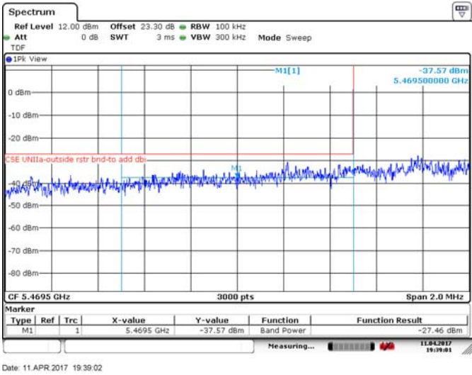
Figure 8.4-165: Lower band edge for FCC, 40 MHz channel, 24 dBi antenna, BPSK
