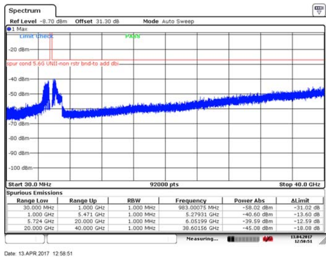
Figure 8.4-196: Spurious emissions outside restricted bands, 40 MHz channel, low channel, 32 dBi antenna, ch1, 256QAM
