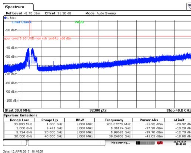
Figure 8.4-172: Spurious emissions outside restricted bands, 10 MHz channel, low channel, 32 dBi antenna, ch1, 256QAM
