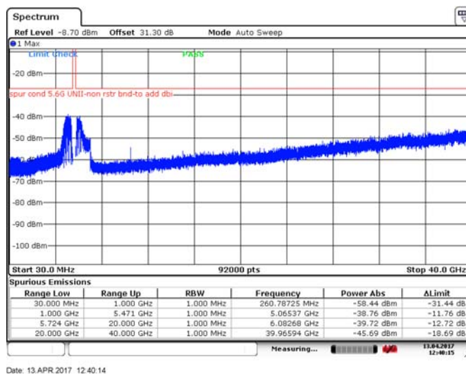
Figure 8.4-192: Spurious emissions outside restricted bands, 20 MHz channel, high channel, 32 dBi antenna, ch1, 256-QAM
