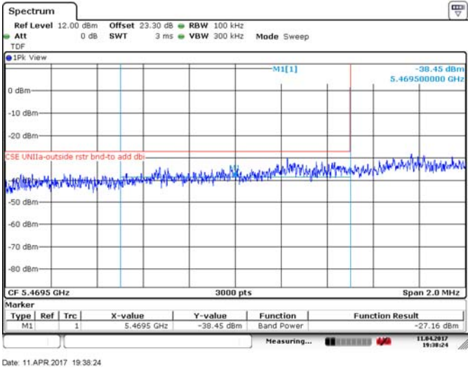
Figure 8.4-167: Lower band edge for FCC, 40 MHz channel, 24 dBi antenna, 256QAM
