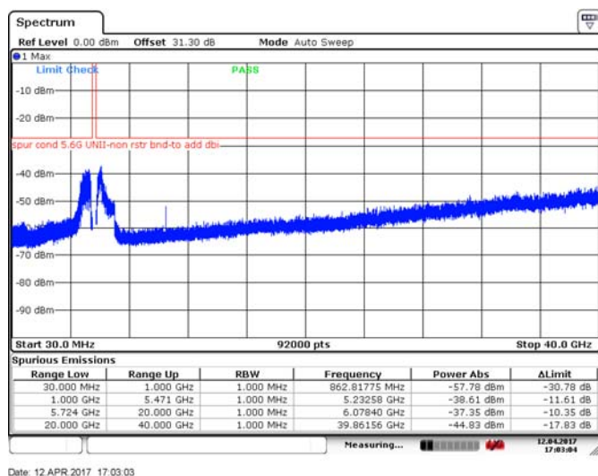
Figure 8.4-185: Spurious emissions outside restricted bands, 20 MHz channel, mid channel, 32 dBi antenna, cho, BPSK
