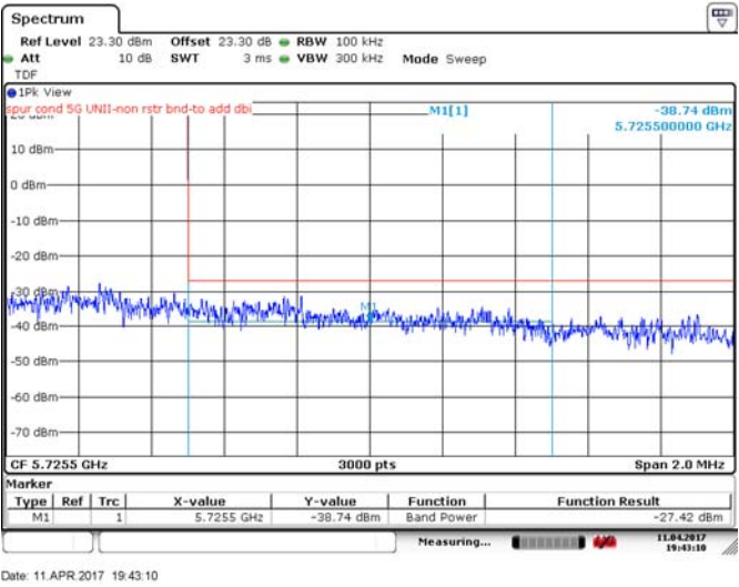
Figure 8.4-166: Upper band edge for FCC, 40 MHz channel, 24 dBi antenna, BPSK
