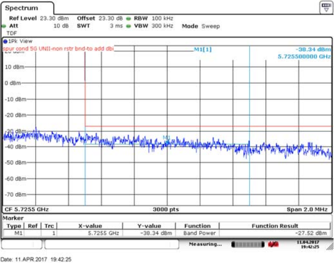
Figure 8.4-168: Upper band edge for FCC, 40 MHz channel, 24 dBi antenna, 256QAM
