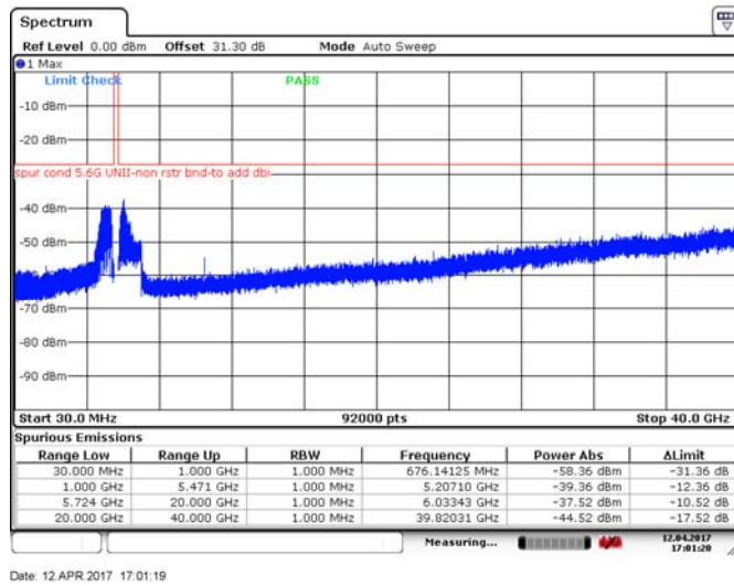
Figure 8.4-183: Spurious emissions outside restricted bands, 20 MHz channel, low channel, 32 dBi antenna, cho, 256QAM
