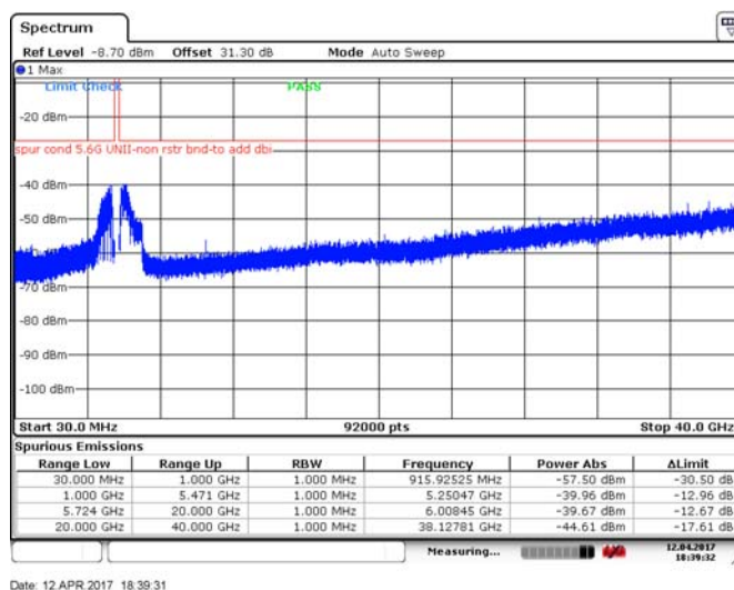
Figure 8.4-170: Spurious emissions outside restricted bands, 10 MHz channel, low channel, 32 dBi antenna, ch1, BPSK
