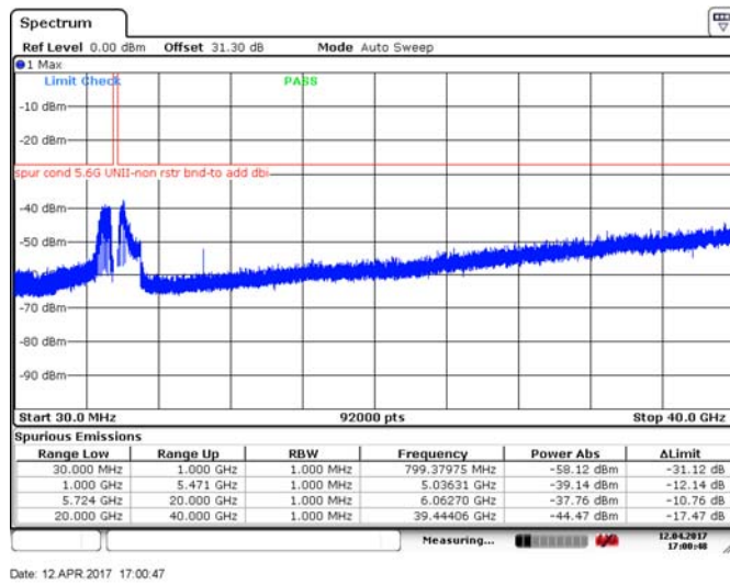
Figure 8.4-181: Spurious emissions outside restricted bands, 20 MHz channel, low channel, 32 dBi antenna, cho, BPSK
