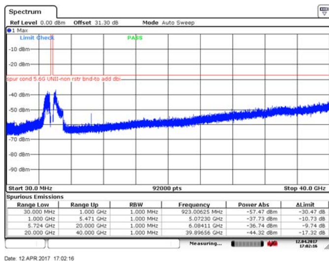
Figure 8.4-187: Spurious emissions outside restricted bands, 20 MHz channel, mid channel, 32 dBi antenna, cho, 256-QAM
