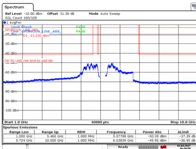
Figure 8.4-216: Average Spurious emissions within restricted bands, 10 MHz channel, mid channel, 32 dBi antenna, cho, 256-QAM
