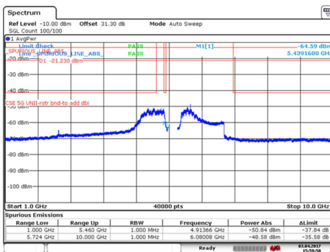
Figure 8.4-214: Average Spurious emissions within restricted bands, 10 MHz channel, mid channel, 32 dBi antenna, cho, BPSK
