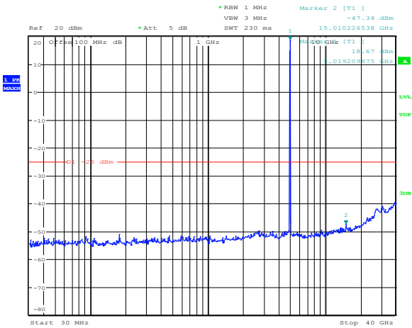
Figure 8.5-32: Spurious emission at low channel, cho, 20 MHz channel
