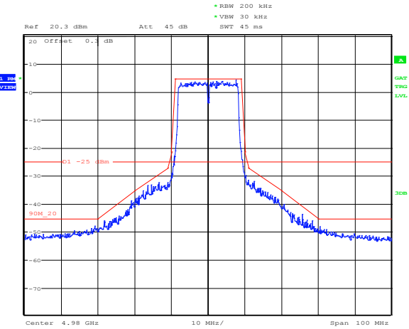
Figure 8.5-17: Emission mask at mid channel, cho, 256-QAM, 20 MHz channel
