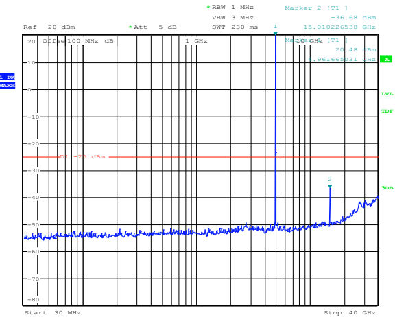
Figure 8.5-25: Emission mask at high channel, ch1, 256-QAM, 20 MHz channel
