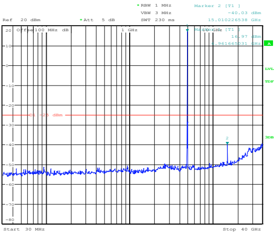
Figure 8.5-33: Spurious emission at mid channel, cho, 20 MHz channel
