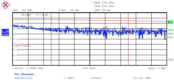
Figure 8.4-331: Upper FCC band edge emissions outside restricted bands at 5850 MHz, 10 MHz channel, 24 dBi antenna, cho, 256-QAM, PTP application
