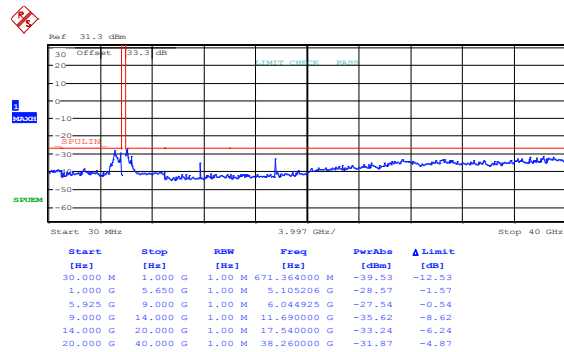
Figure 8.4-275: Spurious emissions outside restricted bands, 10 MHz channel, 24 dBi antenna, low channel, cho, 256-QAM, PTP application
