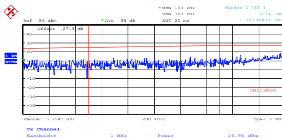
Figure 8.4-304: Spurious emissions outside restricted bands, 40 MHz channel, 24 dBi antenna, ch1, high channel, 256-QAM, PTP application
