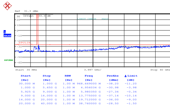
Figure 8.4-296: Spurious emissions outside restricted bands, 40 MHz channel, 24 dBi antenna, ch1, low channel, BPSK, PTP application
