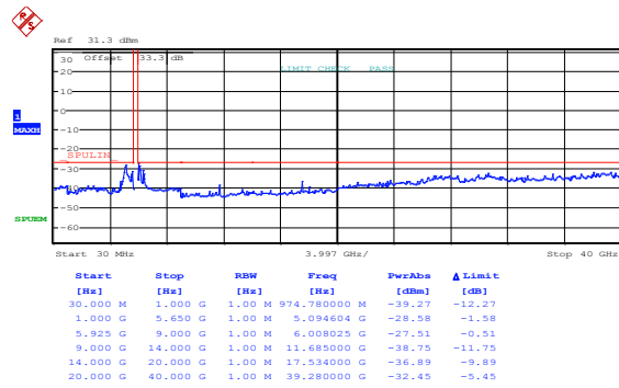
Figure 8.4-287: Spurious emissions outside restricted bands, 20 MHz channel, 24 dBi antenna, low channel, cho, 256-QAM, PTP application
