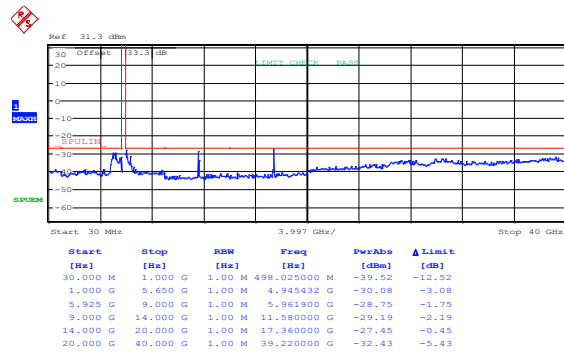
Figure 8.4-271: Spurious emissions outside restricted bands, 10 MHz channel, 24 dBi antenna, high channel, cho, BPSK, PTP application
