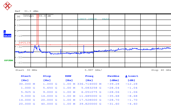
Figure 8.4-272: Spurious emissions outside restricted bands, 10 MHz channel, 24 dBi antenna, ch1, low channel, BPSK, PTP application
