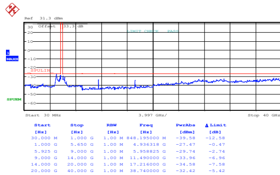
Figure 8.4-300: Spurious emissions outside restricted bands, 40 MHz channel, 24 dBi antenna, cho, mid channel, 256-QAM, PTP application
