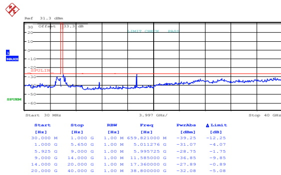
Figure 8.4-280: Spurious emissions outside restricted bands, 10 MHz channel, 24 dBi antenna, ch1, high channel, 256-QAM, PTP application
