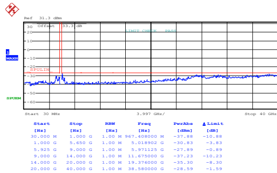
Figure 8.4-299: Spurious emissions outside restricted bands, 40 MHz channel, 24 dBi antenna, low channel, cho, 256-QAM, PTP application
