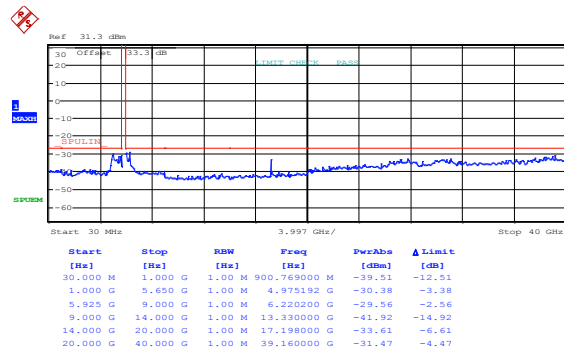
Figure 8.4-279: Spurious emissions outside restricted bands, 10 MHz channel, 24 dBi antenna, mid channel, ch1, 256-QAM, PTP application
