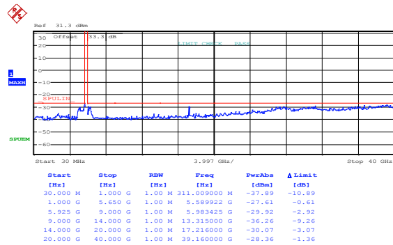
Figure 8.4-291: Spurious emissions outside restricted bands, 20 MHz channel, 24 dBi antenna, mid channel, ch1, 256-QAM, PTP application
