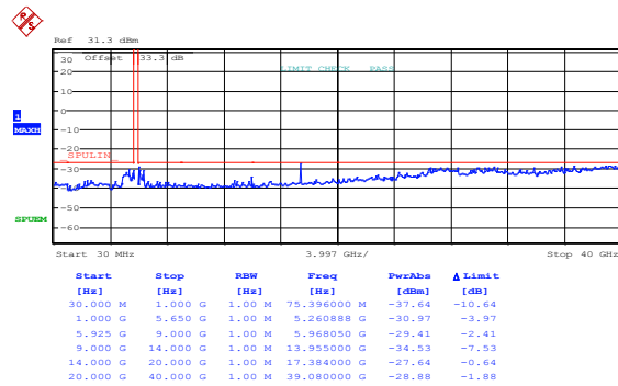
Figure 8.4-292: Spurious emissions outside restricted bands, 20 MHz channel, 24 dBi antenna, ch1, high channel, 256-QAM, PTP application
