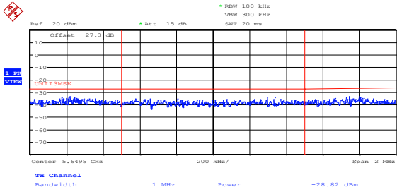
Figure 8.4-315: Lower FCC band edge emissions outside restricted bands at 5650 MHz, 20 MHz channel, 24 dBi antenna, cho, 256-QAM, PTP application
