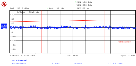
Figure 8.4-408: Lower FCC band edge emissions outside restricted bands at 5725 MHz, 40 MHz channel, 32 dBi antenna, cho, 256-QAM, PTP application
