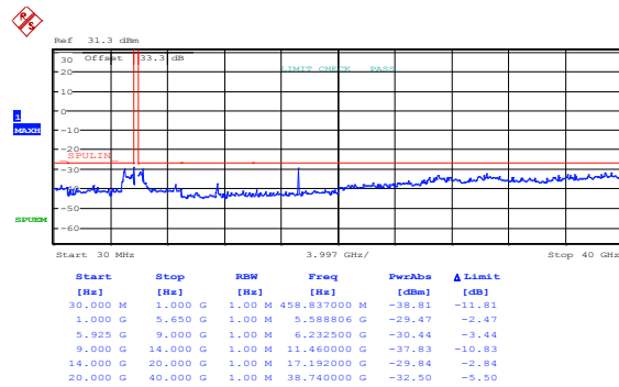
Figure 8.4-276: Spurious emissions outside restricted bands, 10 MHz channel, 24 dBi antenna, cho, mid channel, 256-QAM, PTP application
