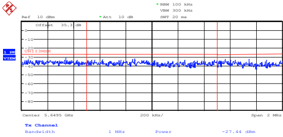
Figure 8.4-407: Lower FCC band edge emissions outside restricted bands at 5650 MHz, 40 MHz channel, 32 dBi antenna, cho, 256-QAM, PTP application
