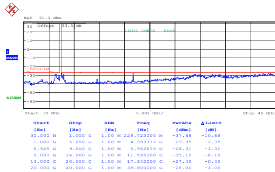
Figure 8.4-295: Spurious emissions outside restricted bands, 40 MHz channel, 24 dBi antenna, high channel, cho, BPSK, PTP application
