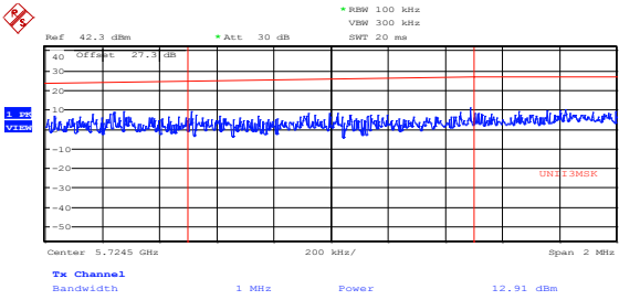
Figure 8.4-316: Lower FCC band edge emissions outside restricted bands at 5725 MHz, 20 MHz channel, 24 dBi antenna, cho, 256-QAM, PTP application
