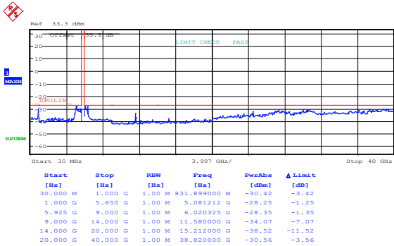
Figure 8.4-352: Upper FCC band edge emissions outside restricted bands at 5925 MHz, 40 MHz channel, 24 dBi antenna, ch1, 256-QAM, PTP application
