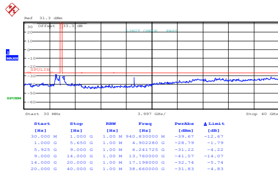
Figure 8.4-288: Spurious emissions outside restricted bands, 20 MHz channel, 24 dBi antenna, cho, mid channel, 256-QAM, PTP application
