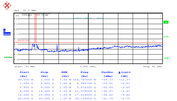
Figure 8.4-283: Spurious emissions outside restricted bands, 20 MHz channel, 24 dBi antenna, high channel, cho, BPSK, PTP application
