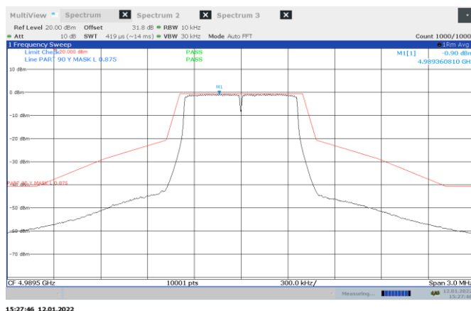
Figure 8.5-7: Emission mask for 0.875 MHz high channel at ch1
