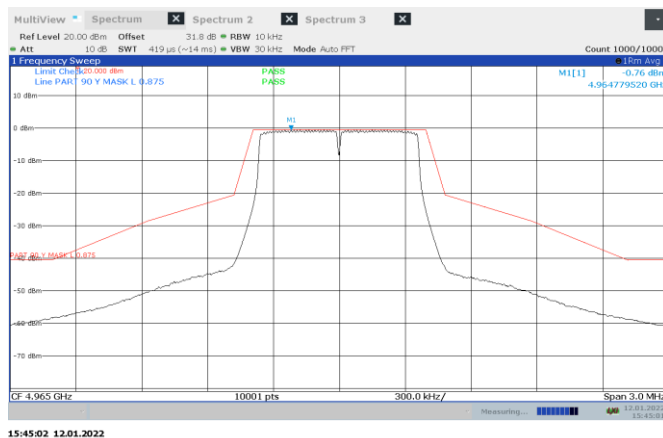
Figure 8.5-5: Emission mask for 0.875 MHz mid channel at ch1
