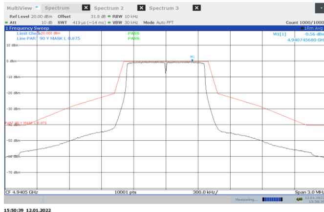
Figure 8.5-3: Emission mask for 0.875 MHz low channel at ch1
