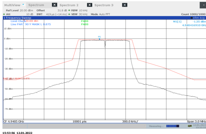
Figure 8.5-2: Emission mask for 0.875 MHz low channel at ch0
