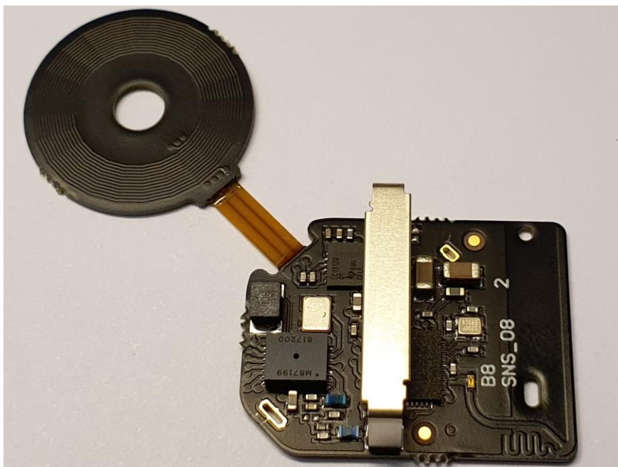
Figure 1 Intuitu circuit board top side
