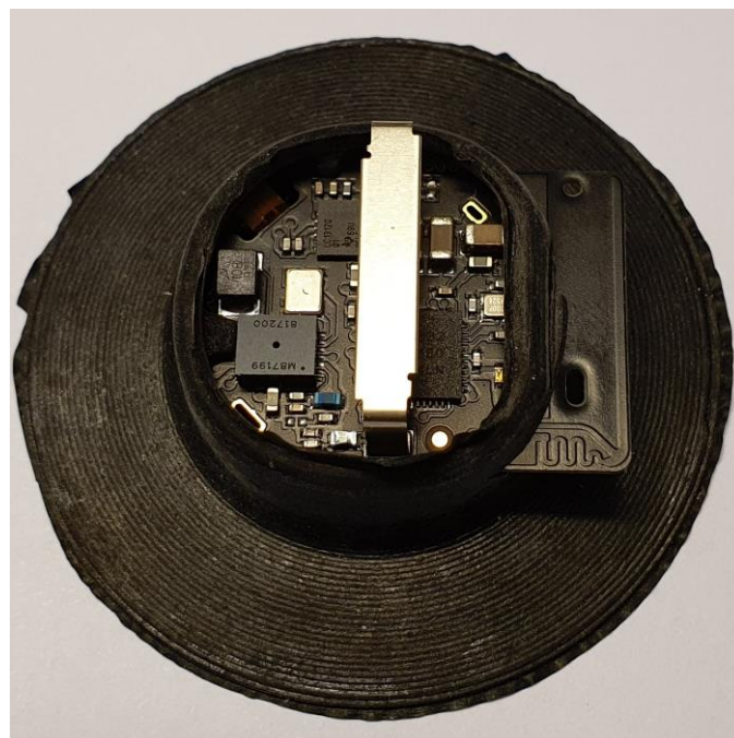
Figure 4 Intuitu circuit board placed on holder
