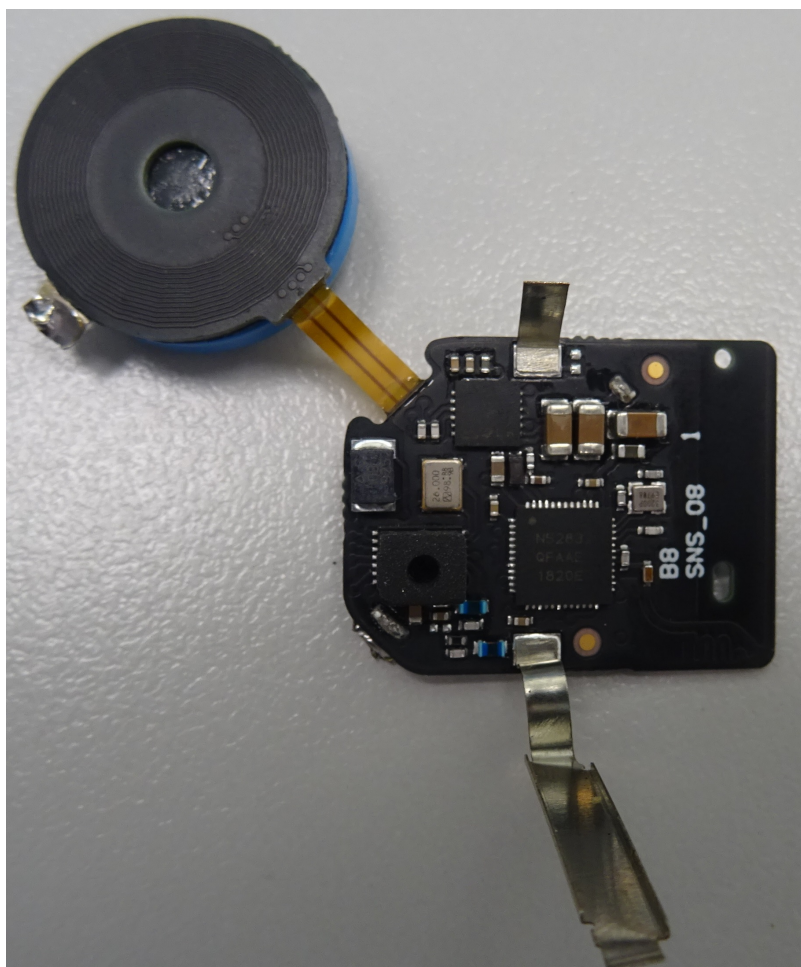
Figure 2 Intuitu circuit board top side without dipole antenna
