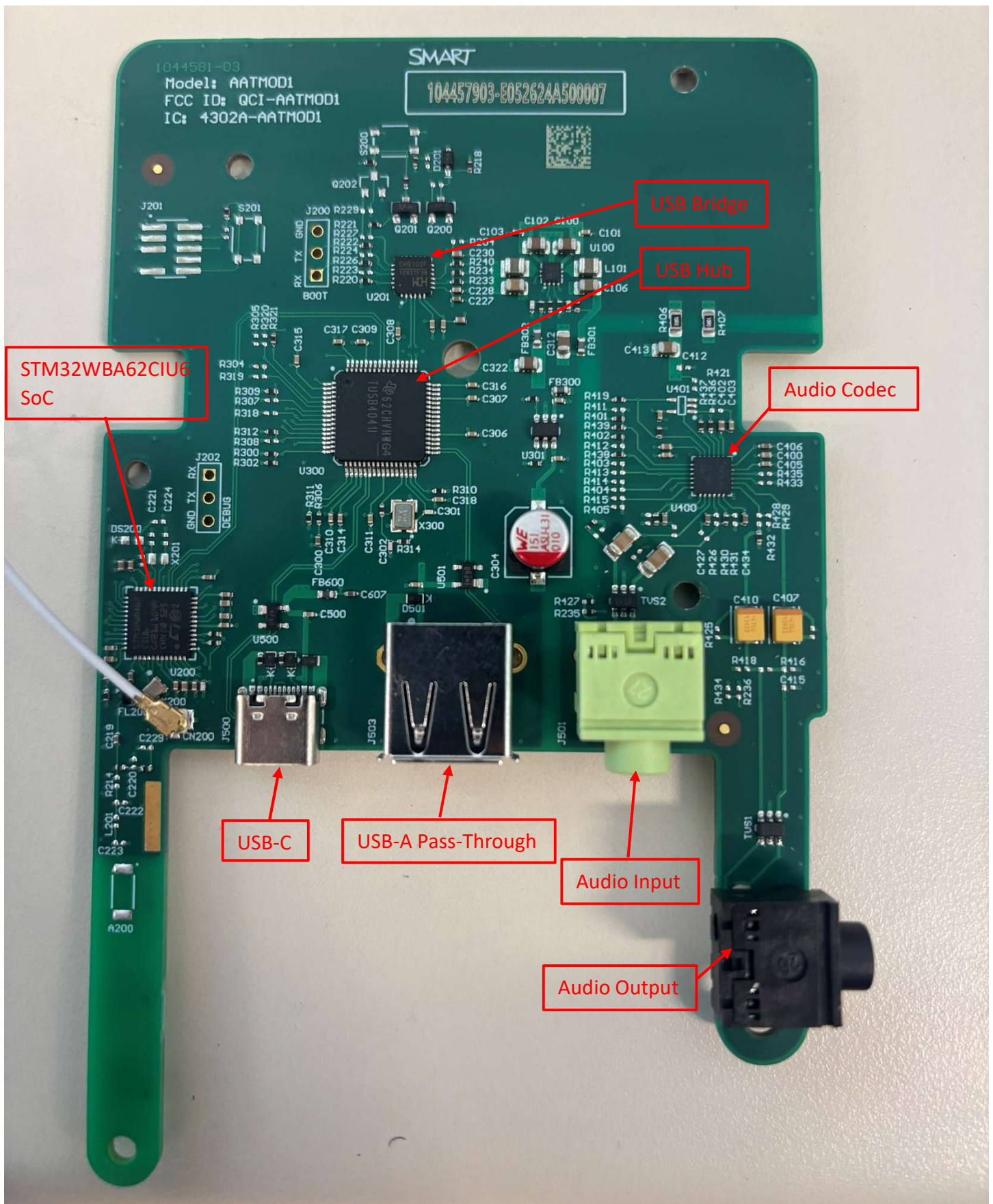
AATMOD1 - Main Board (back)
