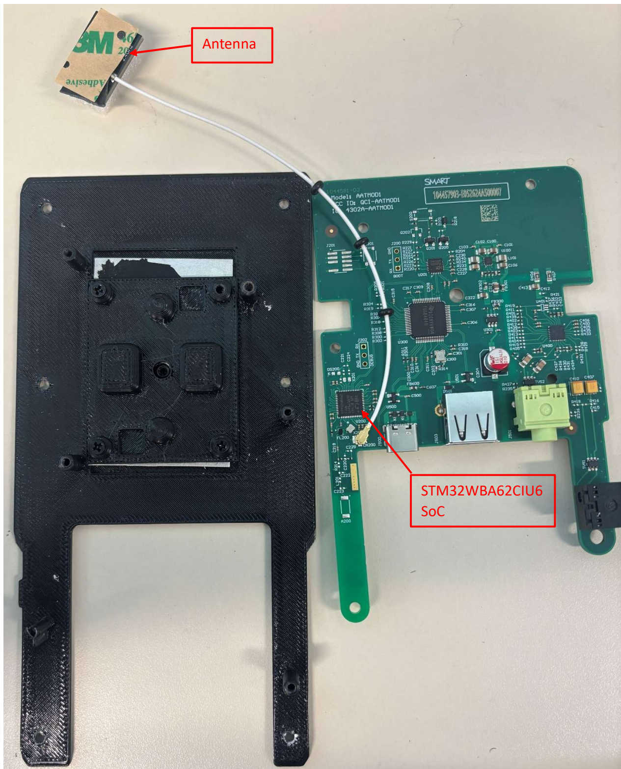
Main Board removed (back)
