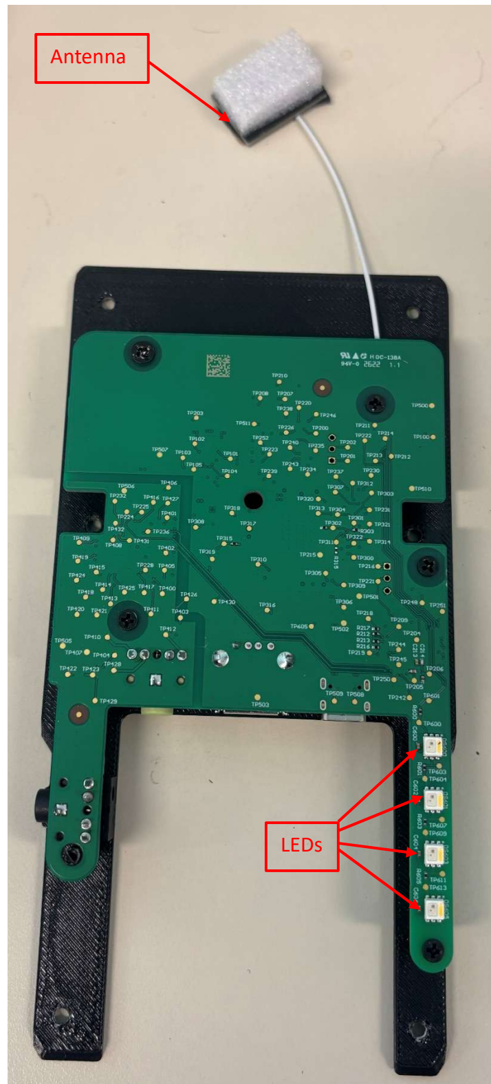
Front Enclosure removed (front)
