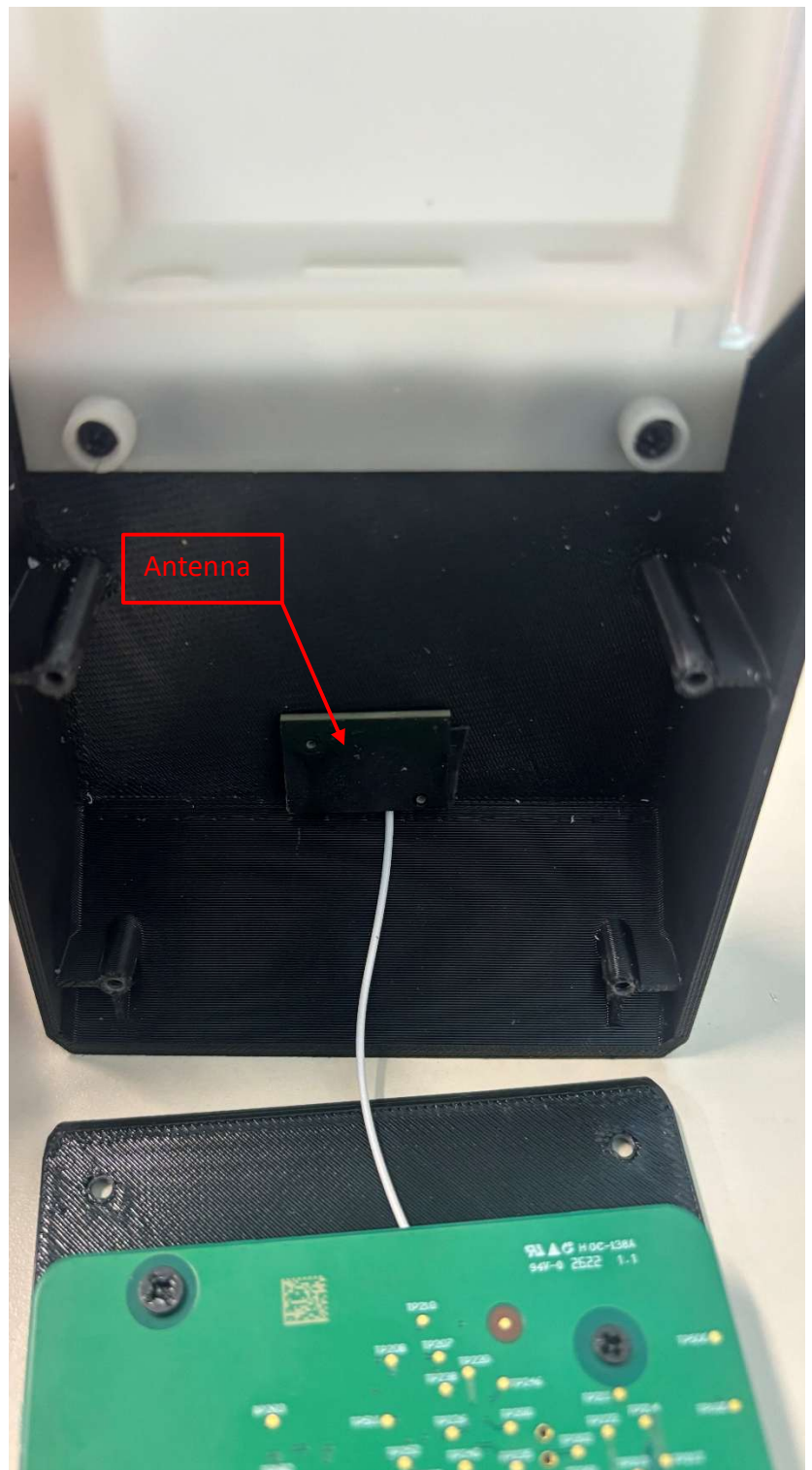
Front Enclosure removed
