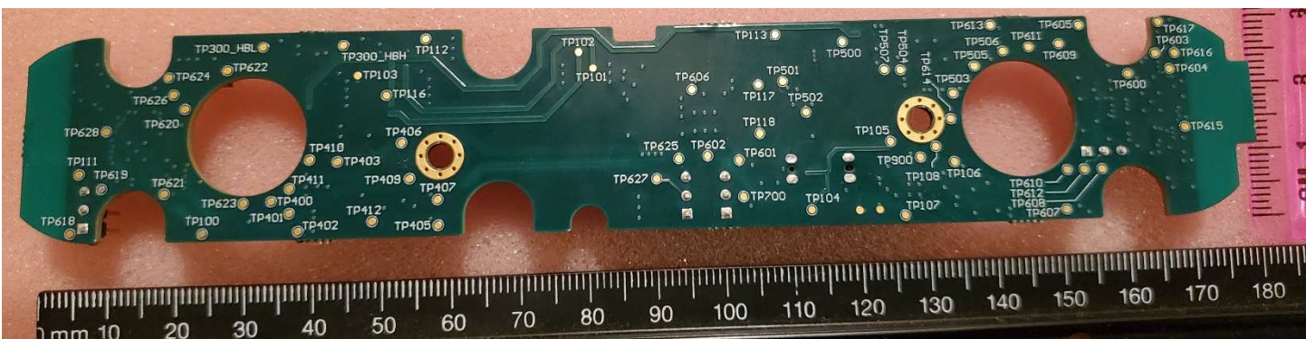
Main board - top
