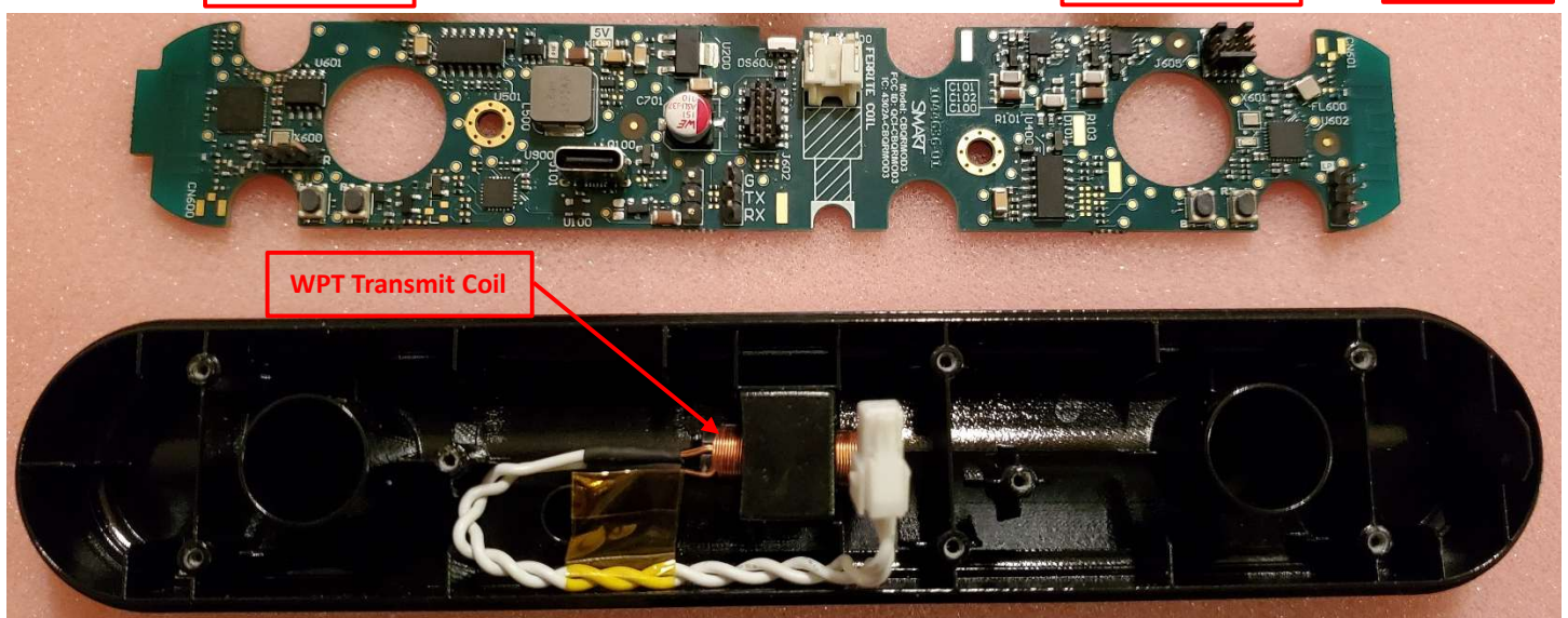
Main board removed
