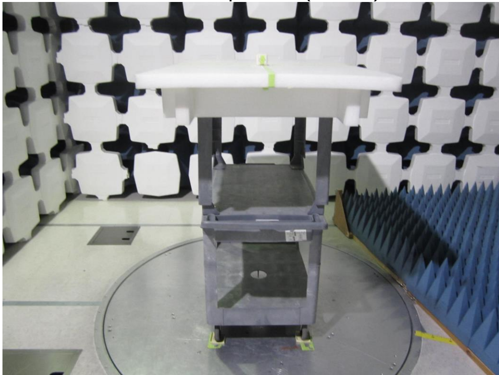
Radiated Spurious (CRX-1)
