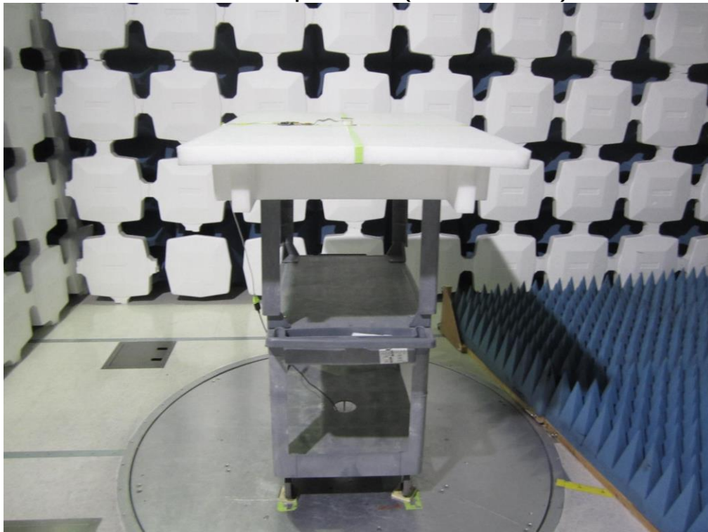
Radiated Spurious (CRXMOD1)
