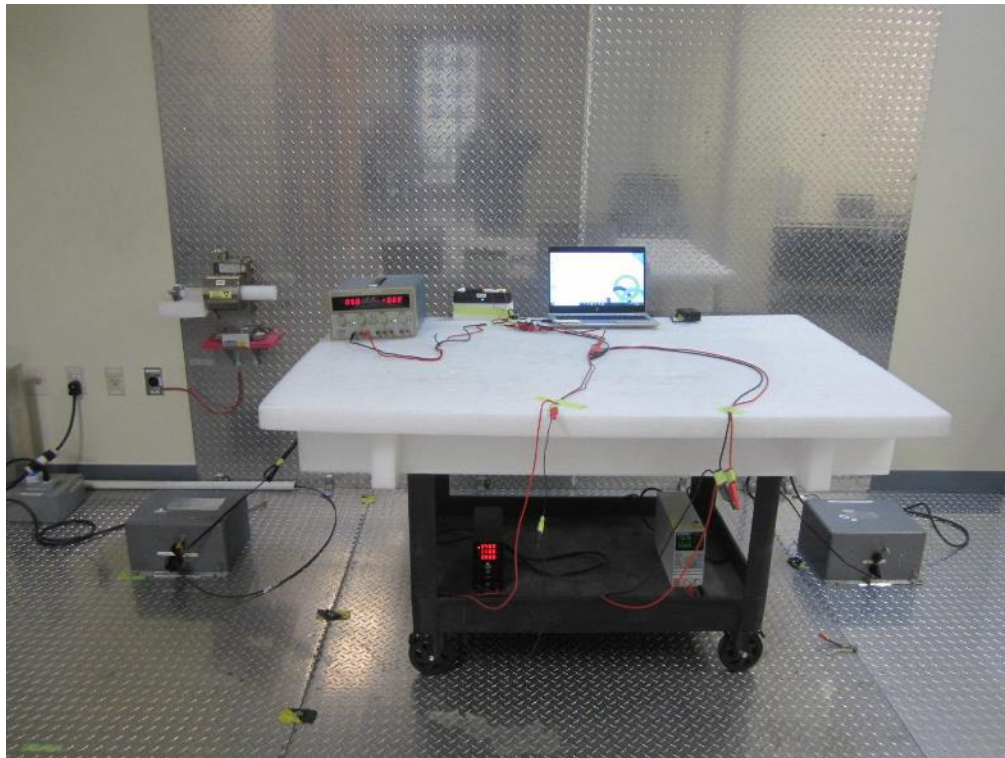
Powerline Conducted Emissions
