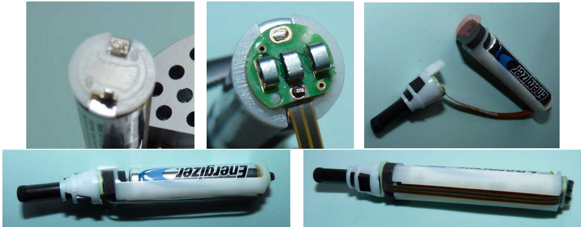
Battery and Pen Tip subassembly
