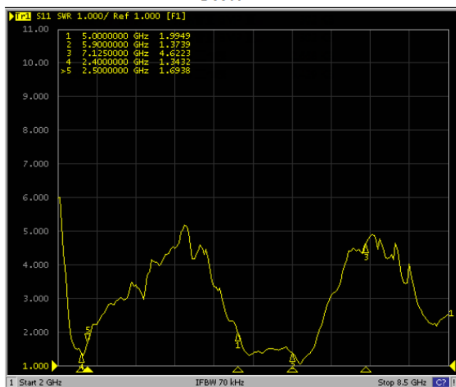
SWR
