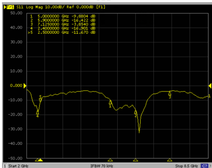
S11
