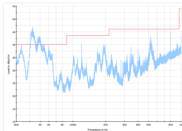
Figure 8.4-11: Radiated spurious emissions for high channel below 1 GHz for restricted band emissions
