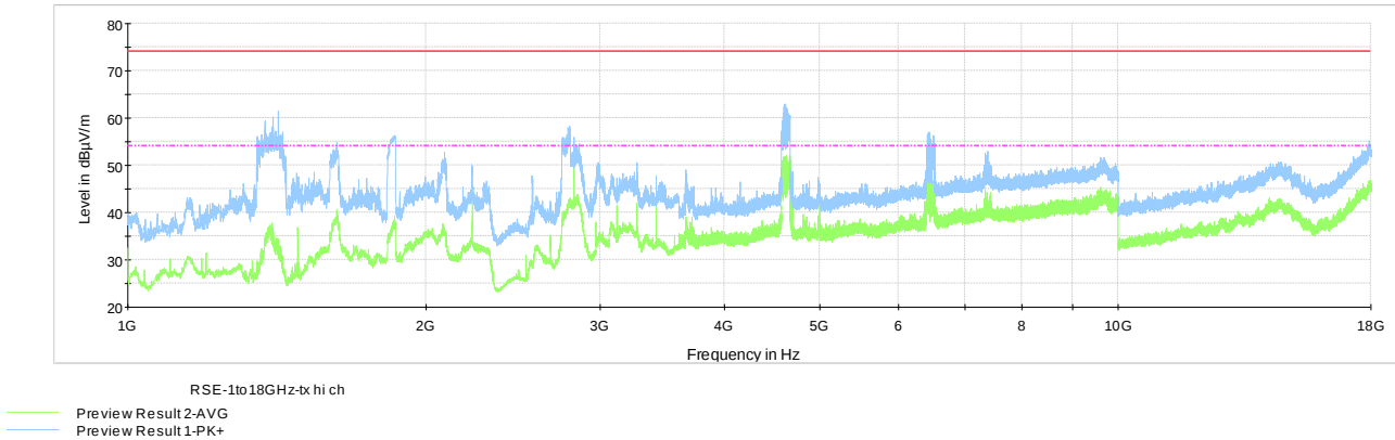
Figure 8.4-14: Radiated spurious emissions for high channel above 1 GHz for restricted band emissions
