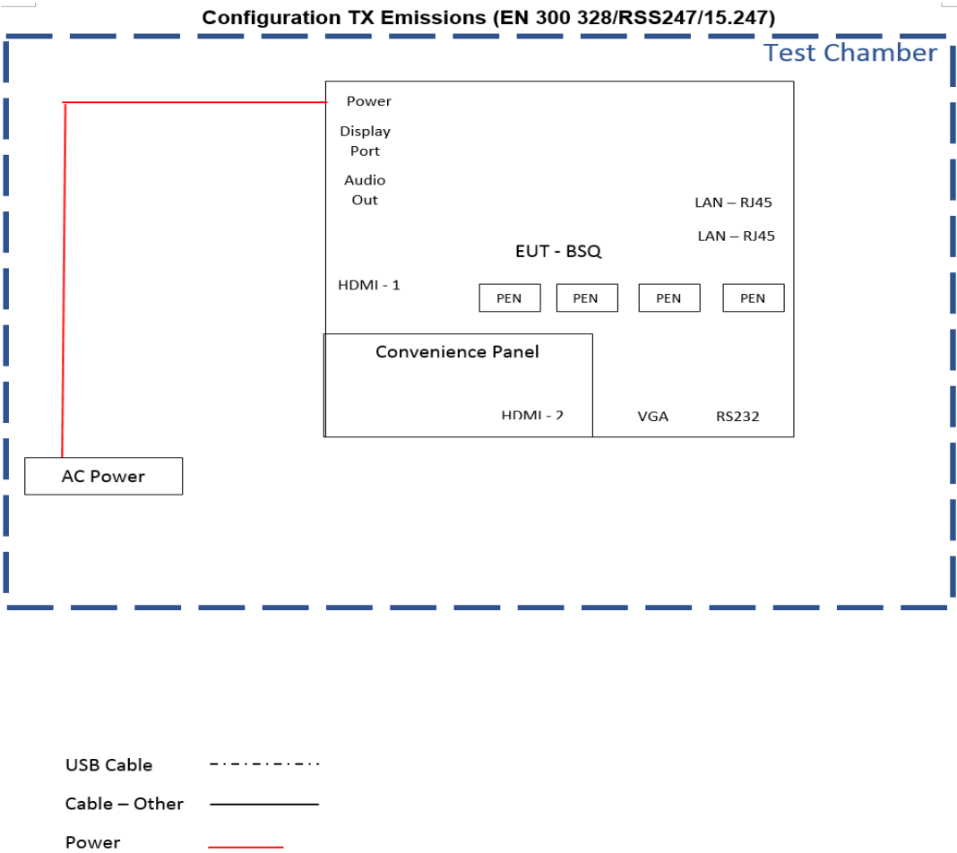
Figure 3.6-1: Setup diagram
