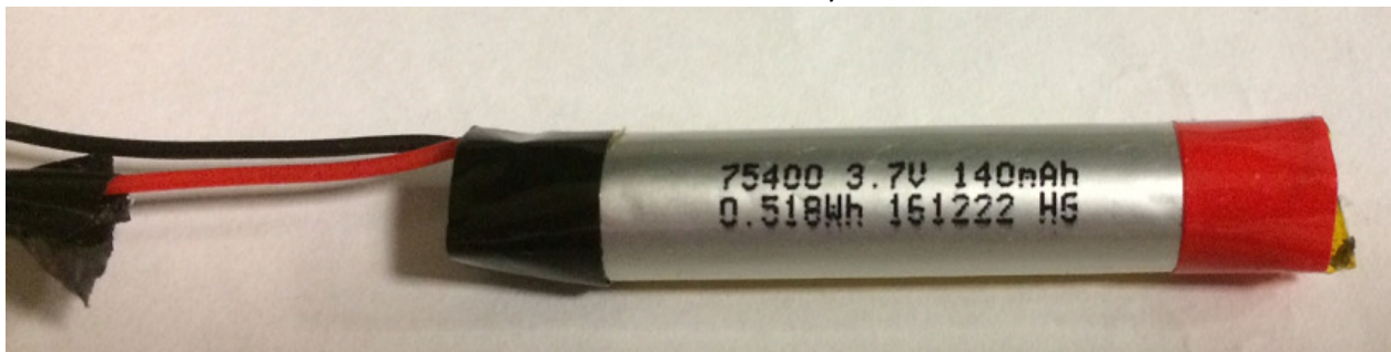
Pen Internal - Battery
