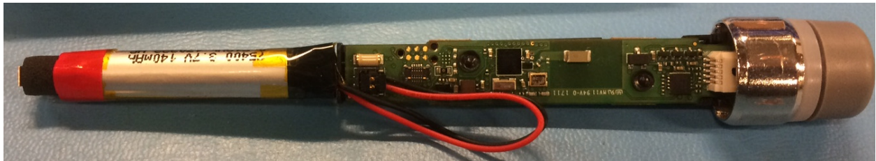
Pen Internal PCB with battery
