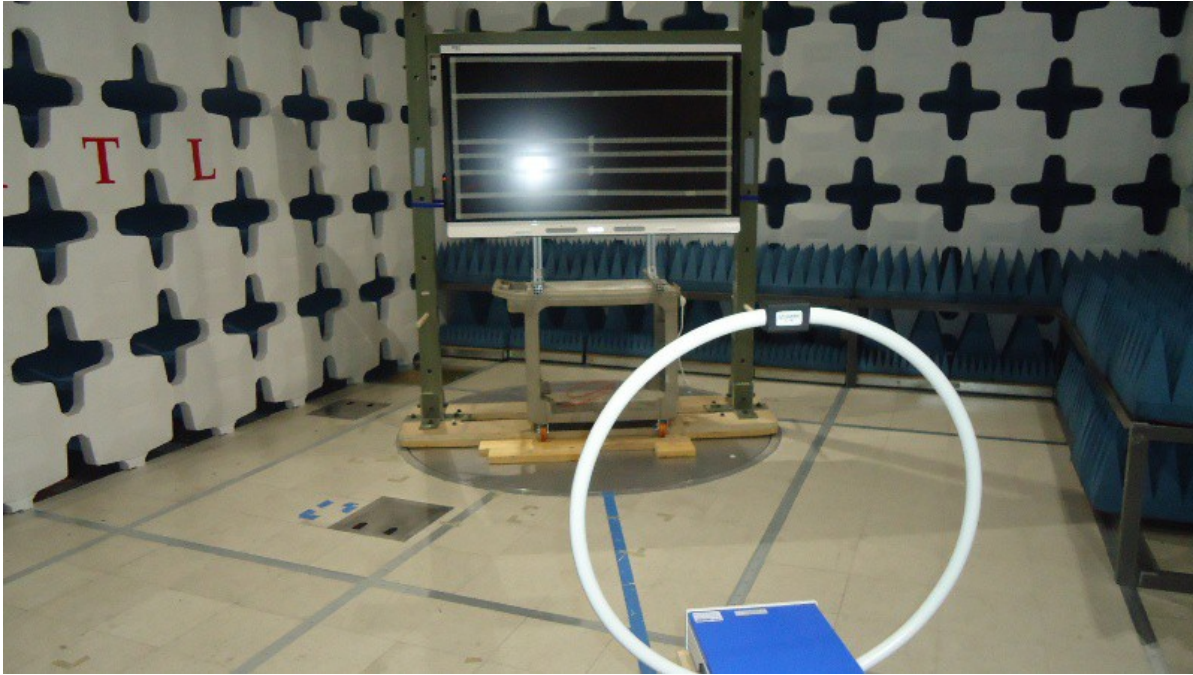
Figure 4.6a - Test Setup - Front View
