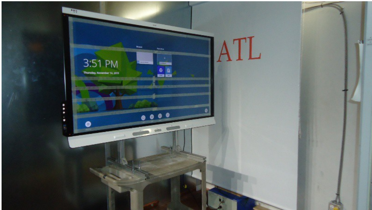
Figure 4.4 - Test Setup - Front View
