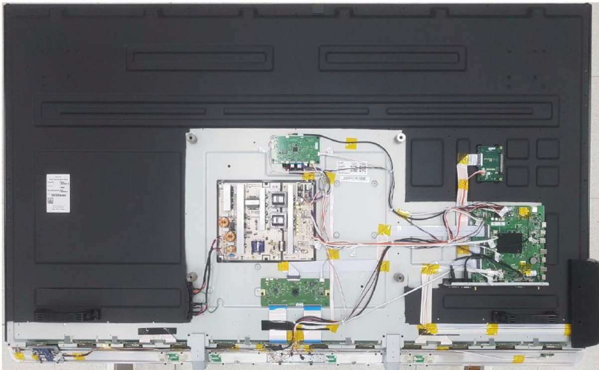
Internal view – Full system
