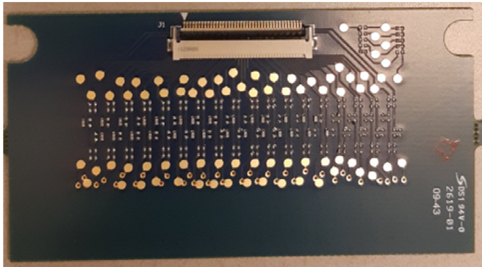
Kansas Matching boards
