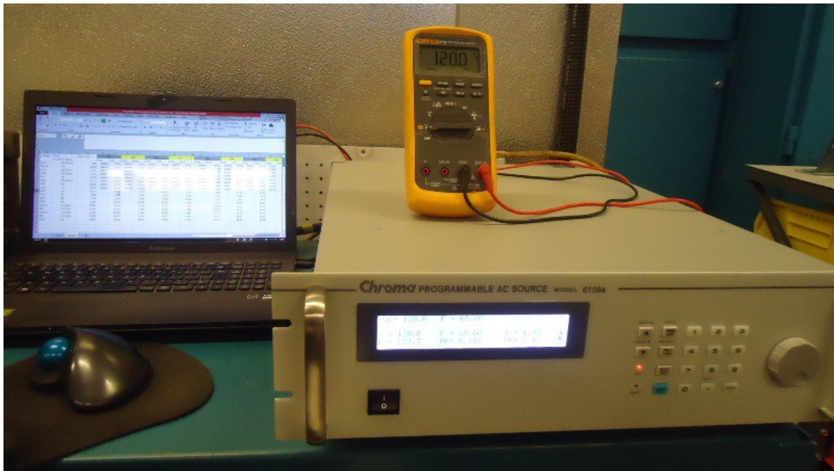
Figure 5.0 - Test Setup - Power system
