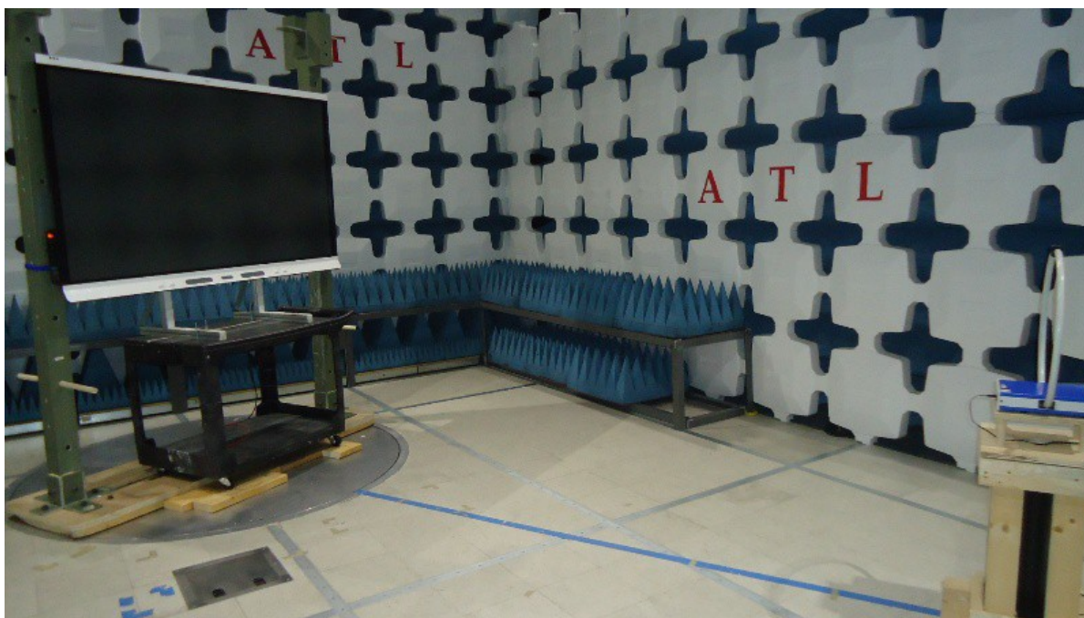
Figure 1.1 - Test Setup - Side View
