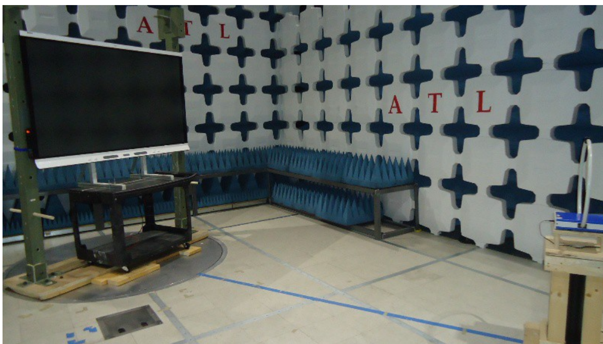
Figure 3.1 - Test Setup - Side View
