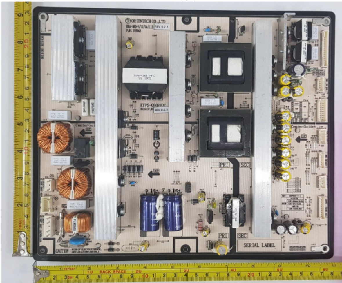
Power Supply
