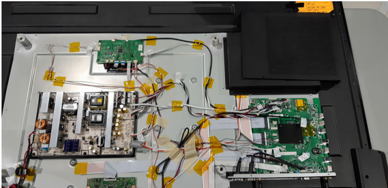
Cable routing – Power Supply, Casper Scaler and Kansas Touch Controller
