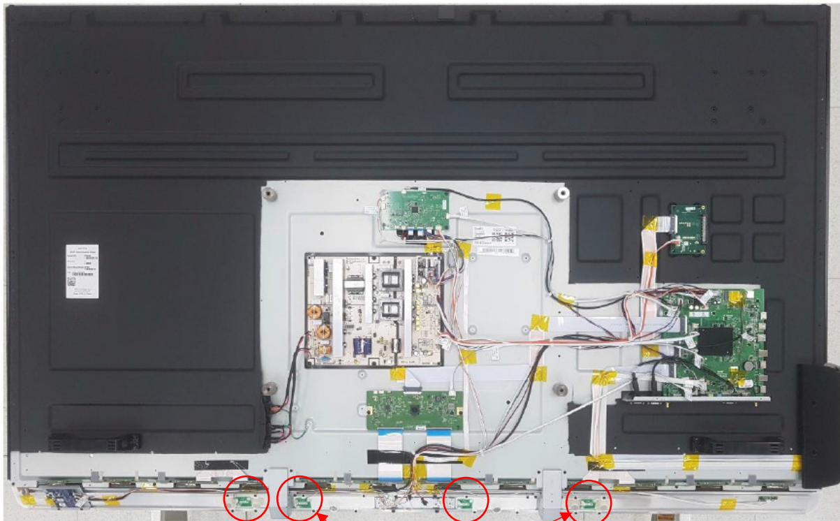
Pen Tray Antenna
