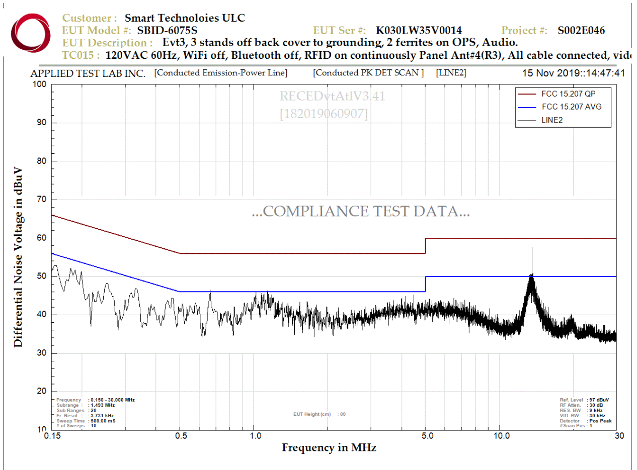
Figure 6.3 - AC Power Line Conducted Emission Scan Line 2 (Line N)
