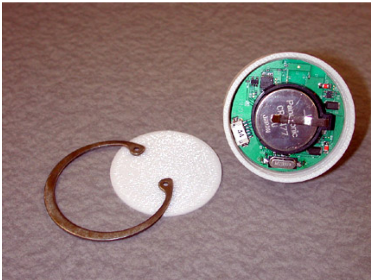
PAL-650 Disassembled
