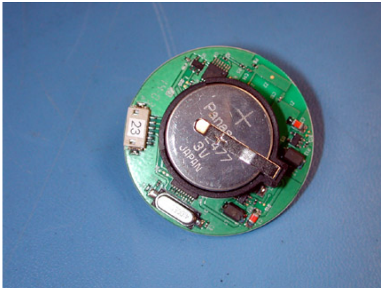
PAL-650 Circuit Side (Battery Installed)
