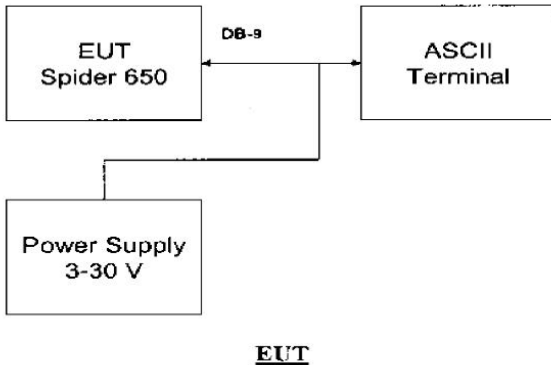
Figure 1. Test Configuration
