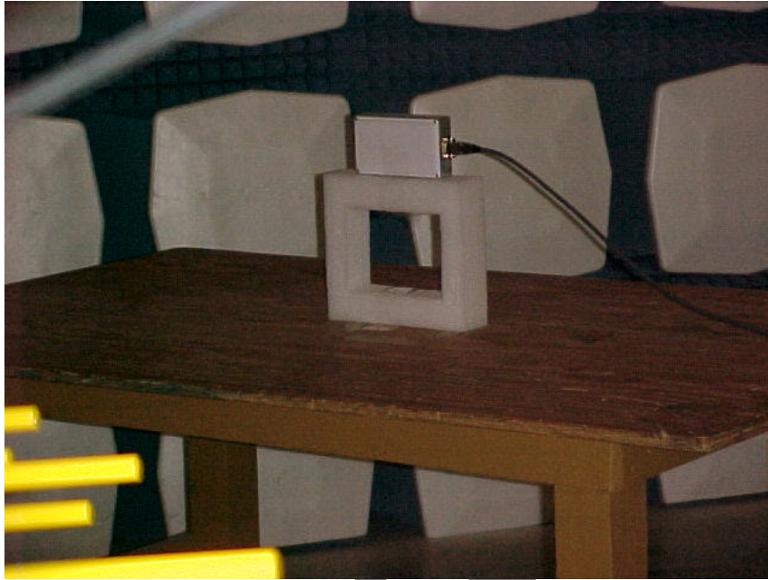
Figure 2. FCC Intentional Radiators Test Setup Photo
