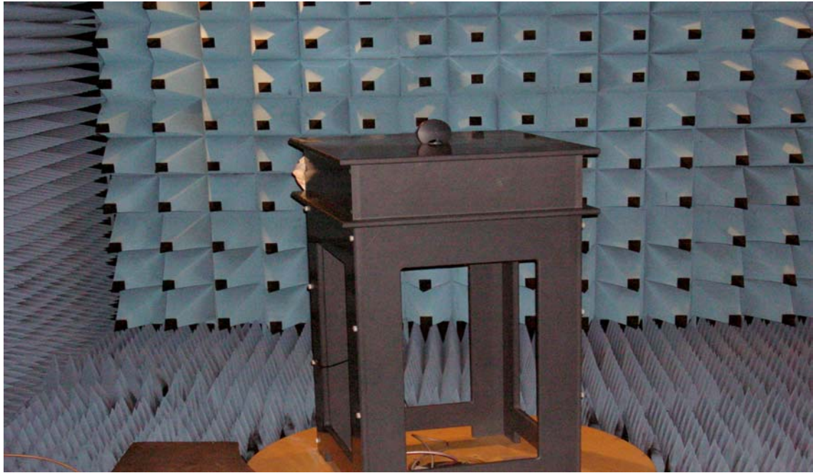
Radiated spurious emissions (1 - 26 GHz)
