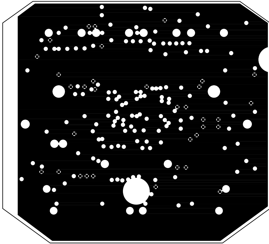
+5V PLANE ISS 2 Q-BOT DISPLAY BOARD \ Lo-Q PLC
