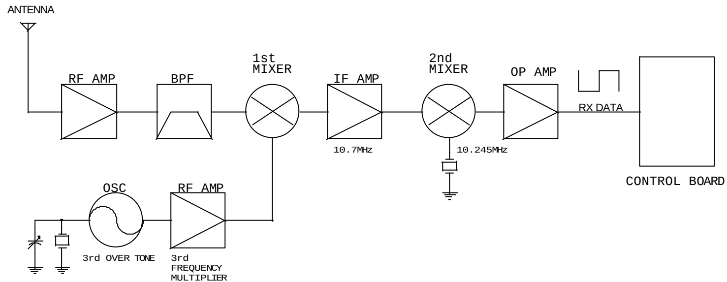
<RX BOARD BLOCK DIAGRAM>
