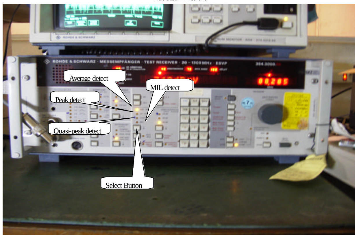
Radiated Emissions
