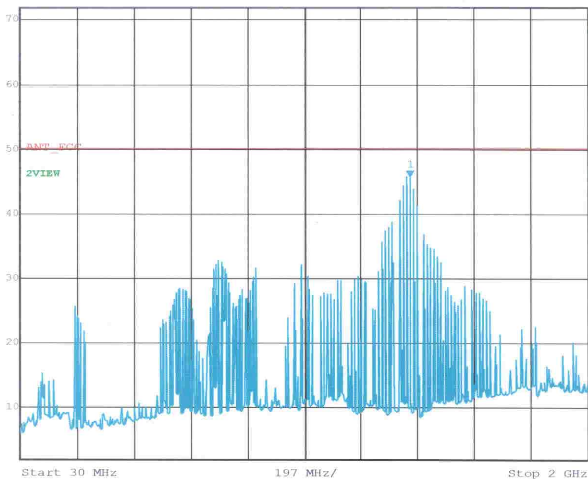
< Fig 6. Antenna power conduction result >
