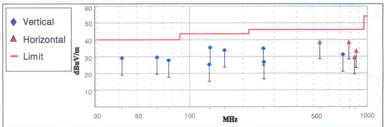
&lt; Fig 5. Radiated emission result _ Digital &gt;
