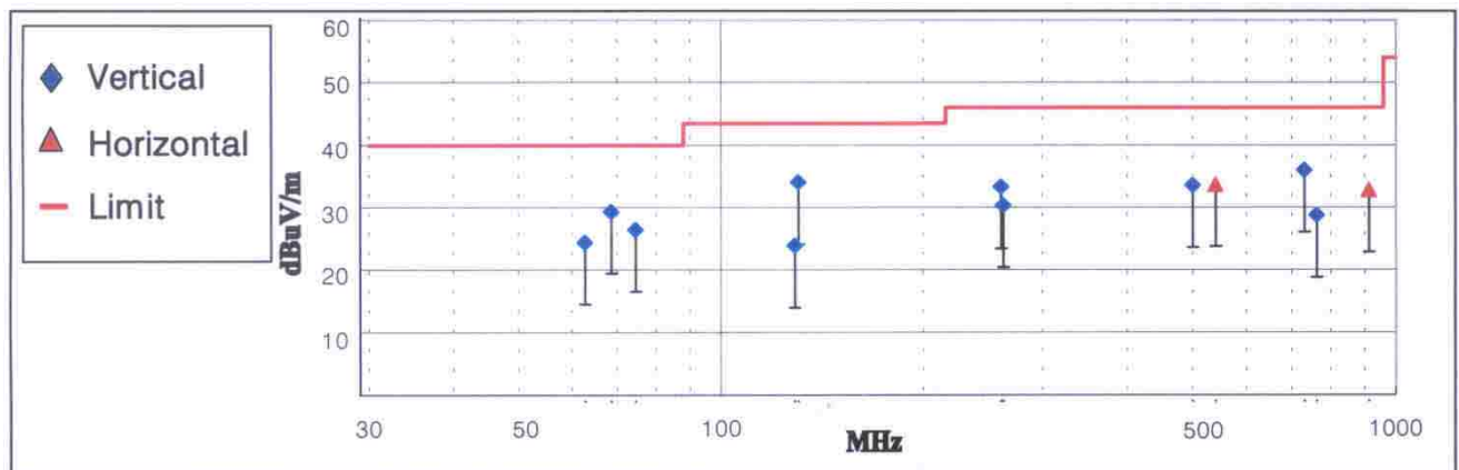
< Fig 4. Radiated emission result _ Analog >
