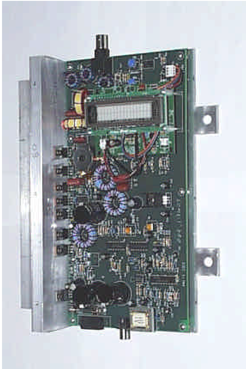
Photo 4. Top View of Board
