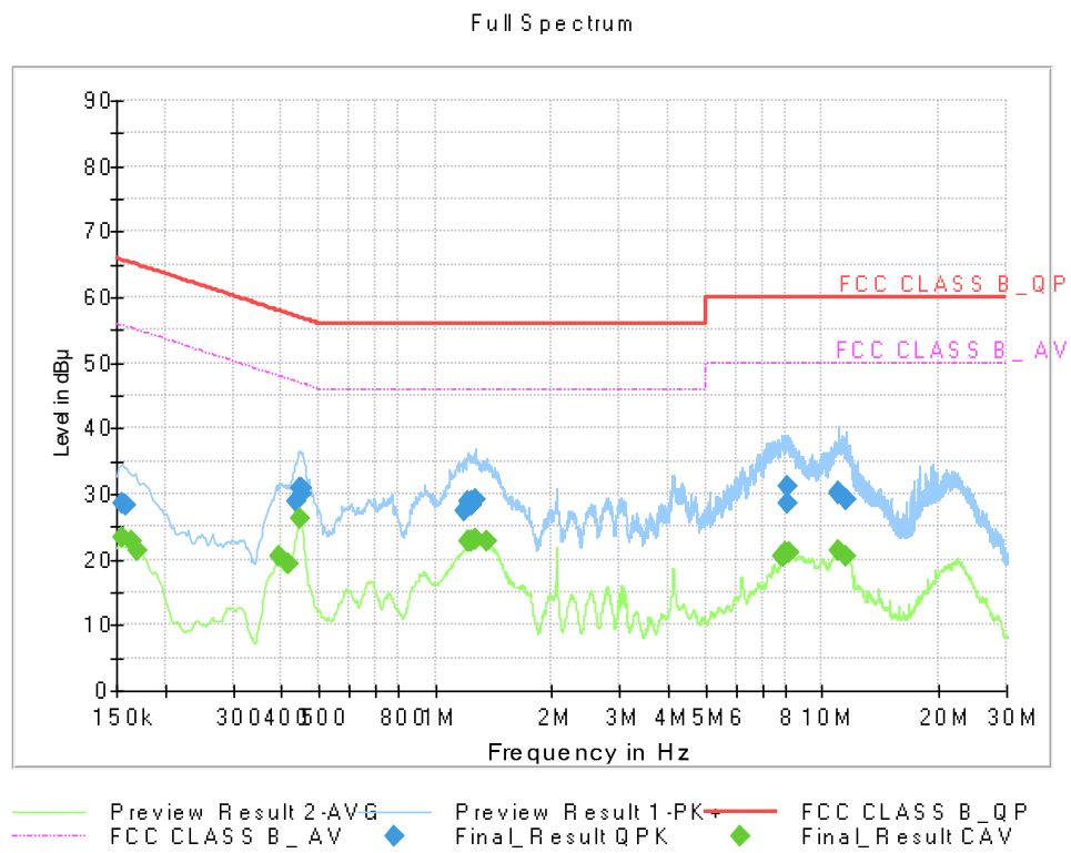
Figure 3: Conducted Emission (0.15 to 30) MHz, PRINTER(USB DATA) mode, Line (L1)
