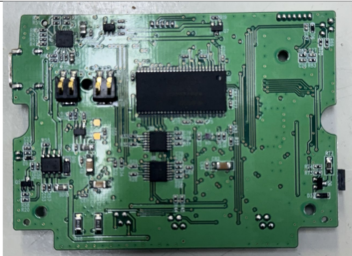
(Main_PCB Rear)
