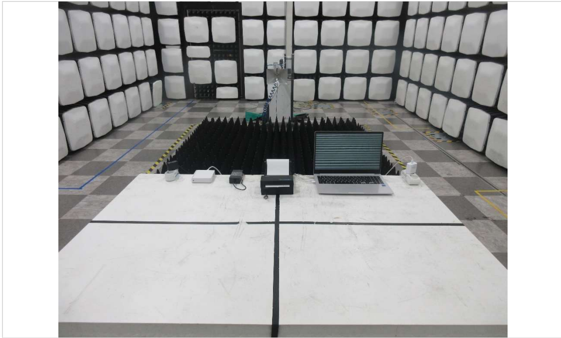
[USB+Printing+Cutting Mode]
