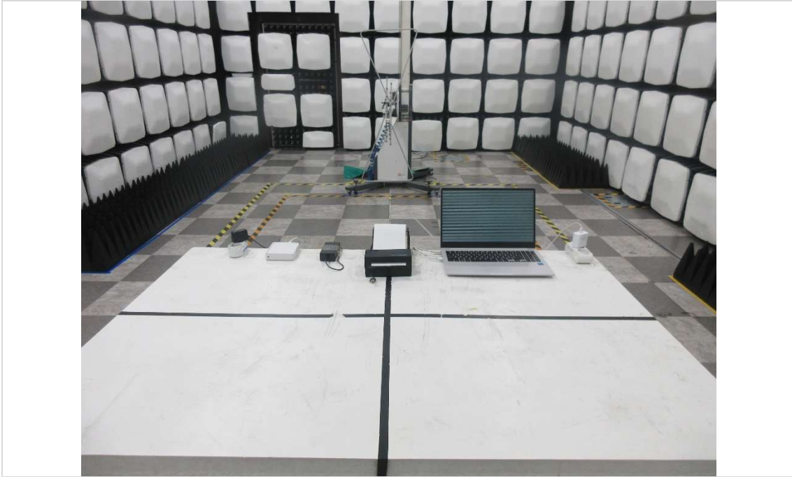
[USB+Printing+Cutting Mode]
