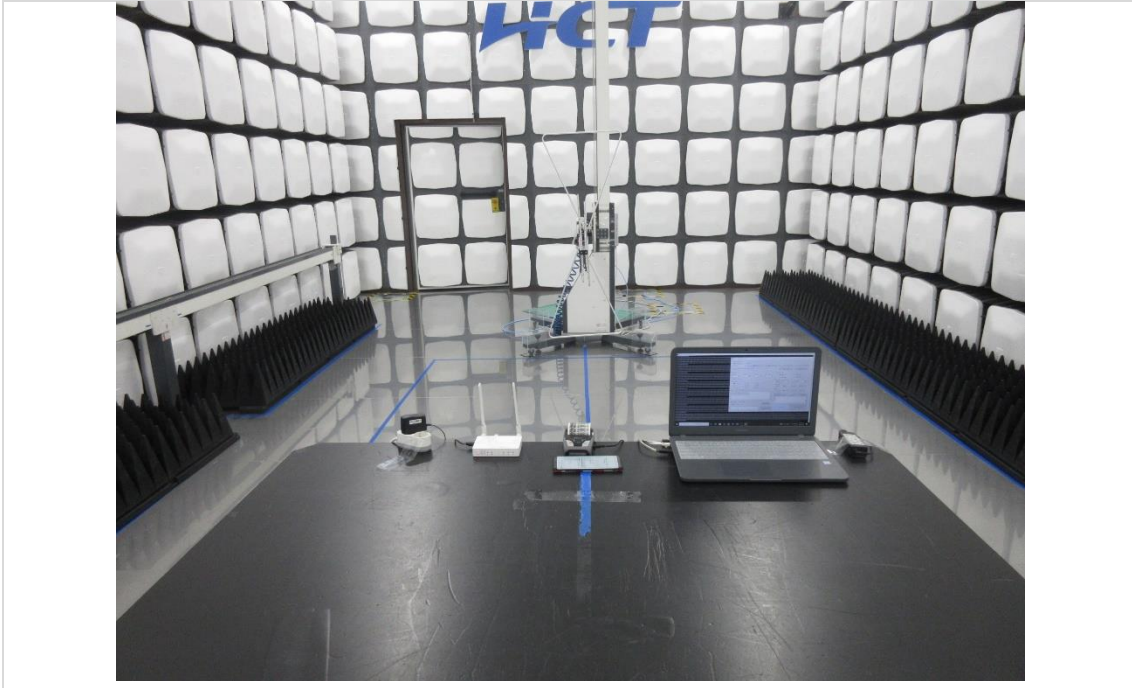
USB(Printer) + MSR + Battery Mode
