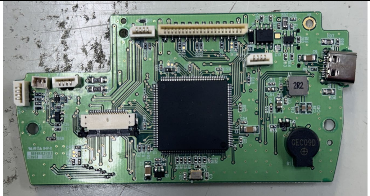
(Main_Front)
