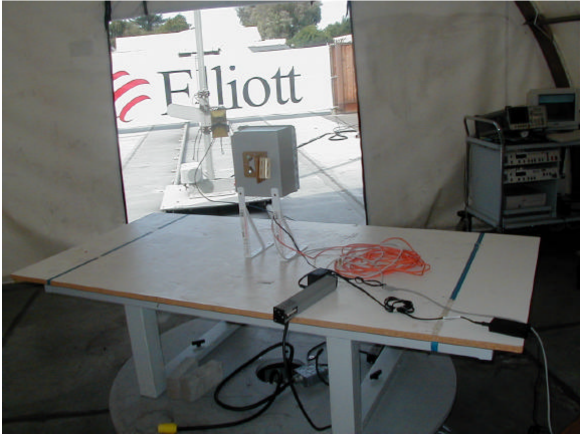
Radiated Emission above 1 GHz Test Setup
