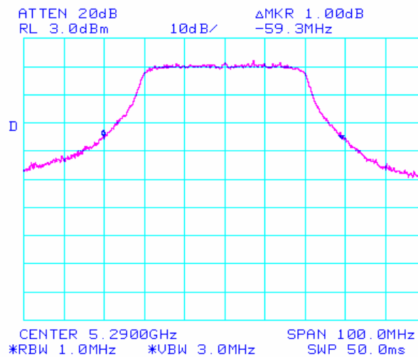
Plot 12: 26dB Bandwidth – 50MHz Center (23dBi)
