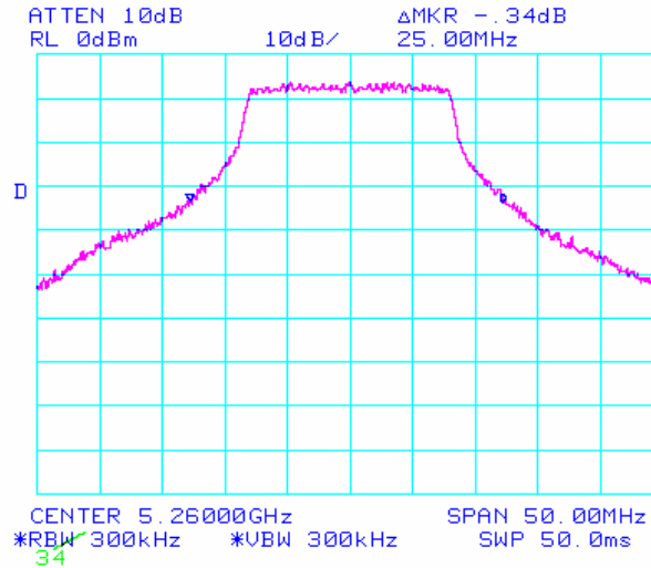
Plot 7: 26dB Bandwidth – 20MHz Low (23dBi)
