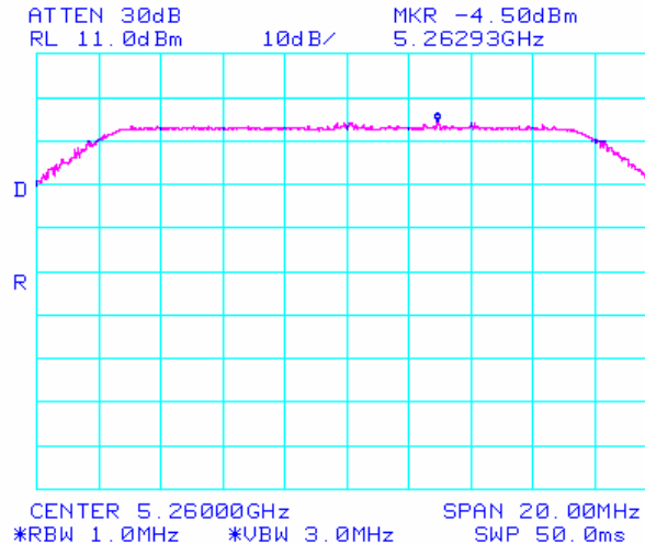
Plot 81: Peak Power Spectral Density (RSS210) – 20MHz Low (28dBi)
