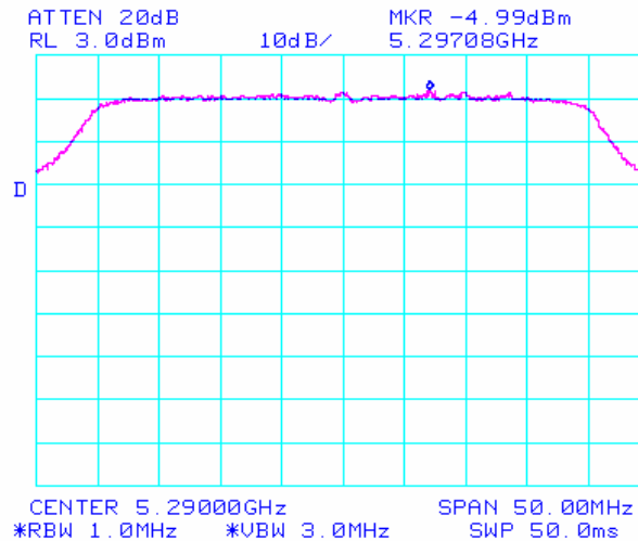
Plot 80: Peak Power Spectral Density (RSS210) – 50MHz Center (23dBi)
