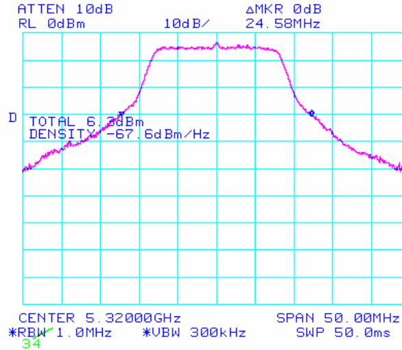
Plot 43: Peak Power – 20MHz Hi (23dBi)
