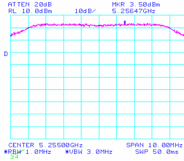
Plot 72: Peak Power Spectral Density (RSS210) – 10MHz Low (23dBi)
