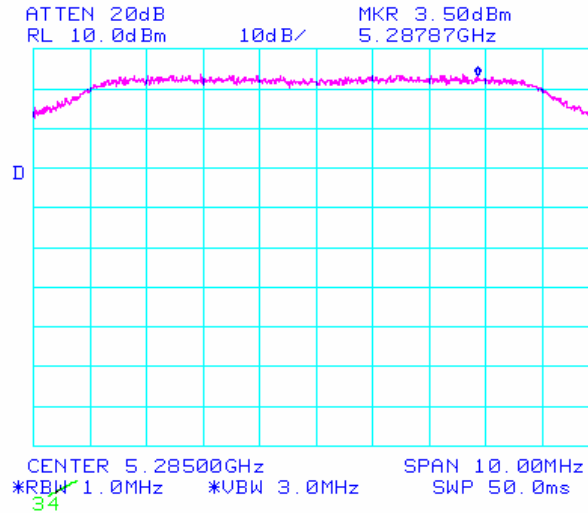
Plot 73: Peak Power Spectral Density (RSS210) – 10MHz Mid (23dBi)
