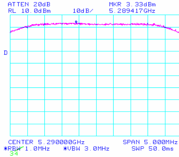
Plot 70: Peak Power Spectral Density (RSS210) – 5MHz Mid (23dB)
