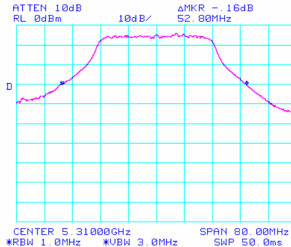
Plot 11: 26dB Bandwidth – 40MHz Hi (23dBi)
