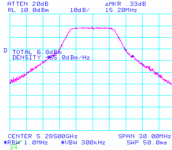
Plot 39: Peak Power – 10MHz Mid (23dBi)
