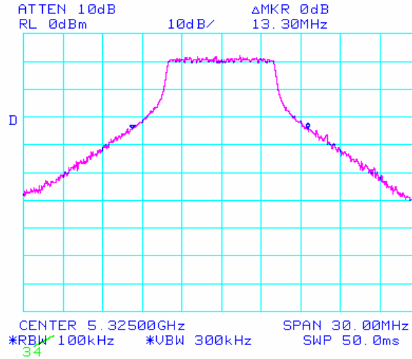
Plot 6: 26dB Bandwidth – 10MHz Hi (23dBi)
