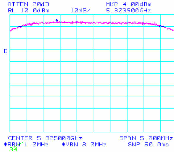
Plot 71: Peak Power Spectral Density (RSS210) – 5MHz Hi (23dB)
