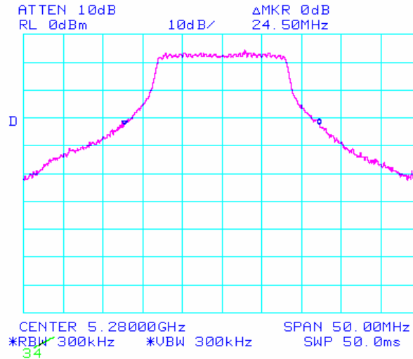
Plot 8: 26dB Bandwidth – 20MHz Mid (23dBi)
