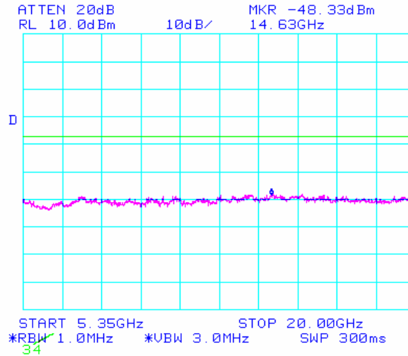
Plot 105: Conducted Spurious Emissions – 5MHz Mid (1/2)
