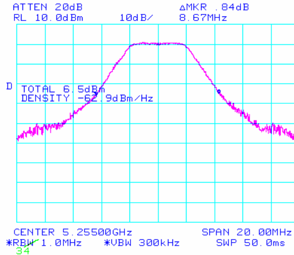
Plot 35: Peak Power – 5MHz Low (23dBi)
