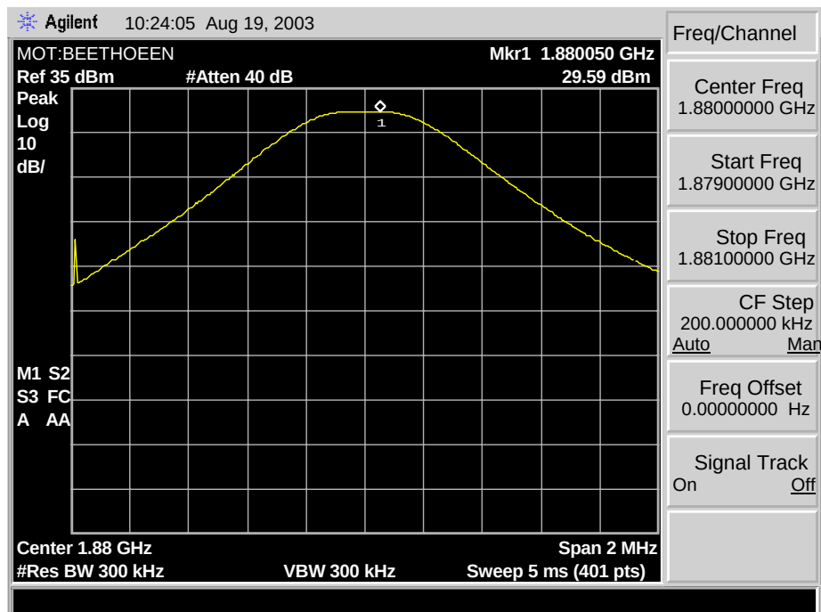
1900 GSM Reference Plot
