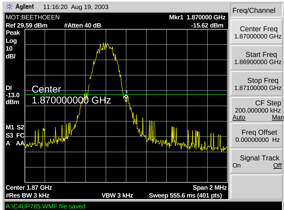
GSM 1900 D Max. Block Edge
