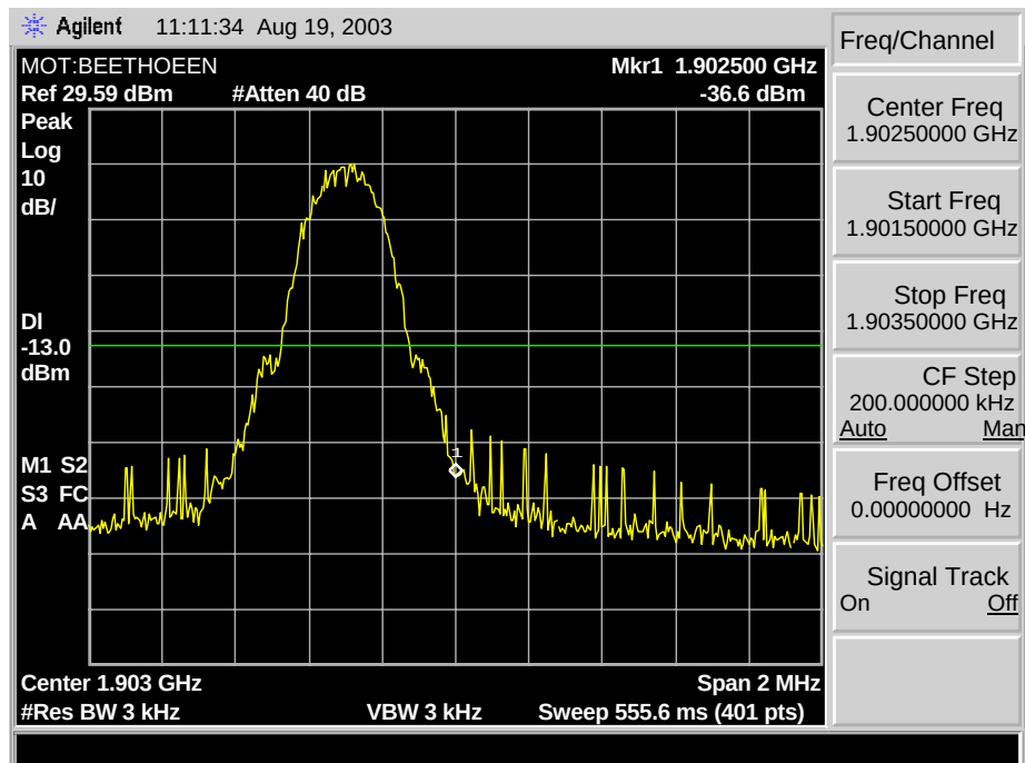
GSM 1900 C, C2, C3 Max Block Edge
