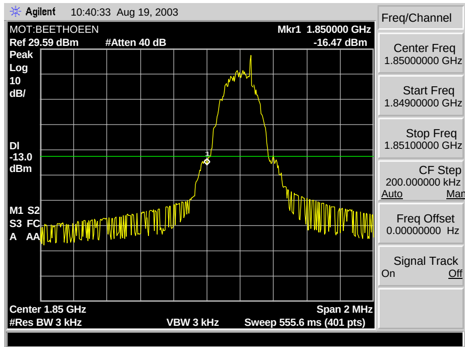
GSM 1900 A Min Block Edge
