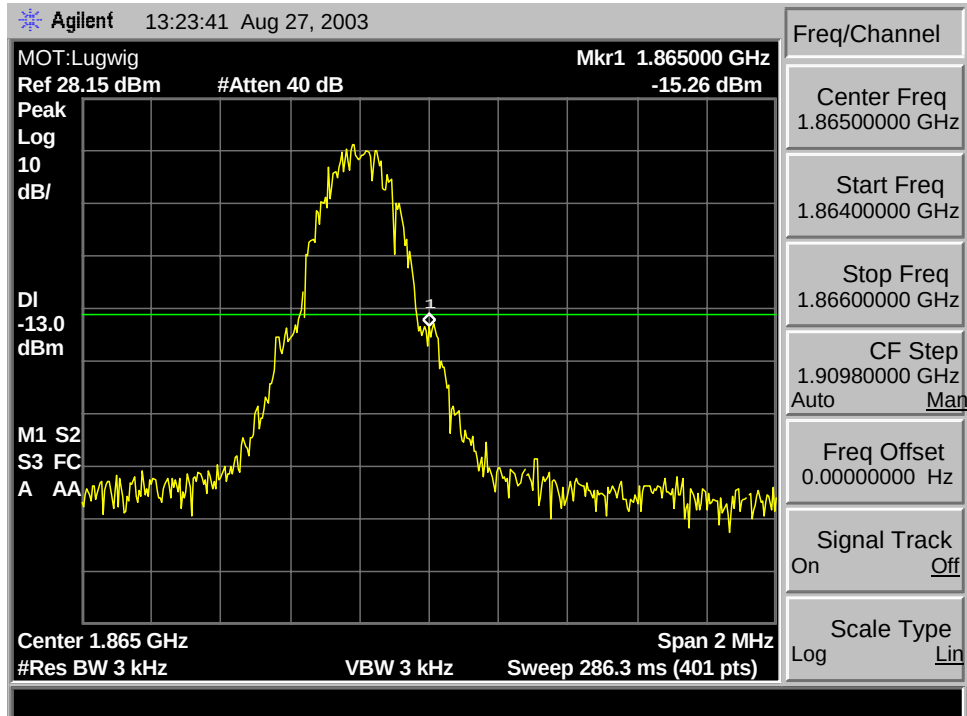
GSM 1900 A Max. Block Edge
