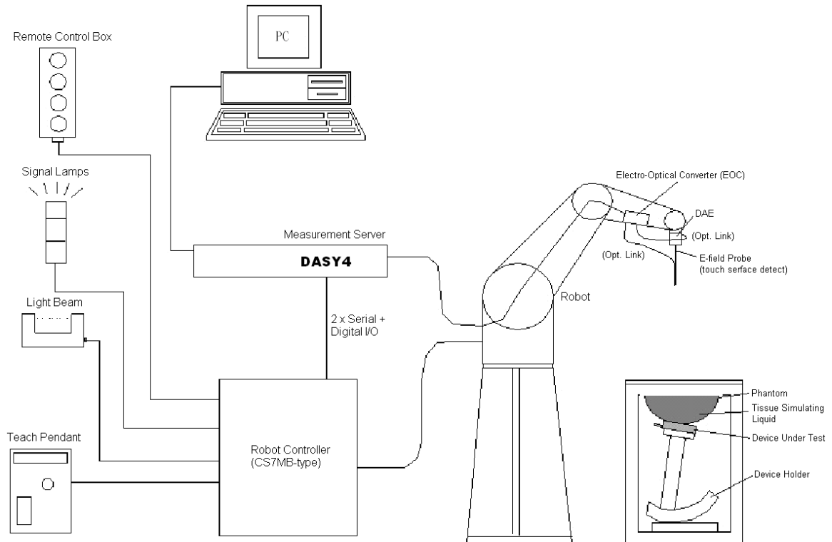
Fig. 5.1 DASY4 system
