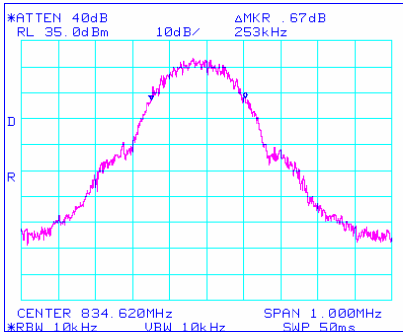
Plot 5 Occupied Bandwidth Test Results
