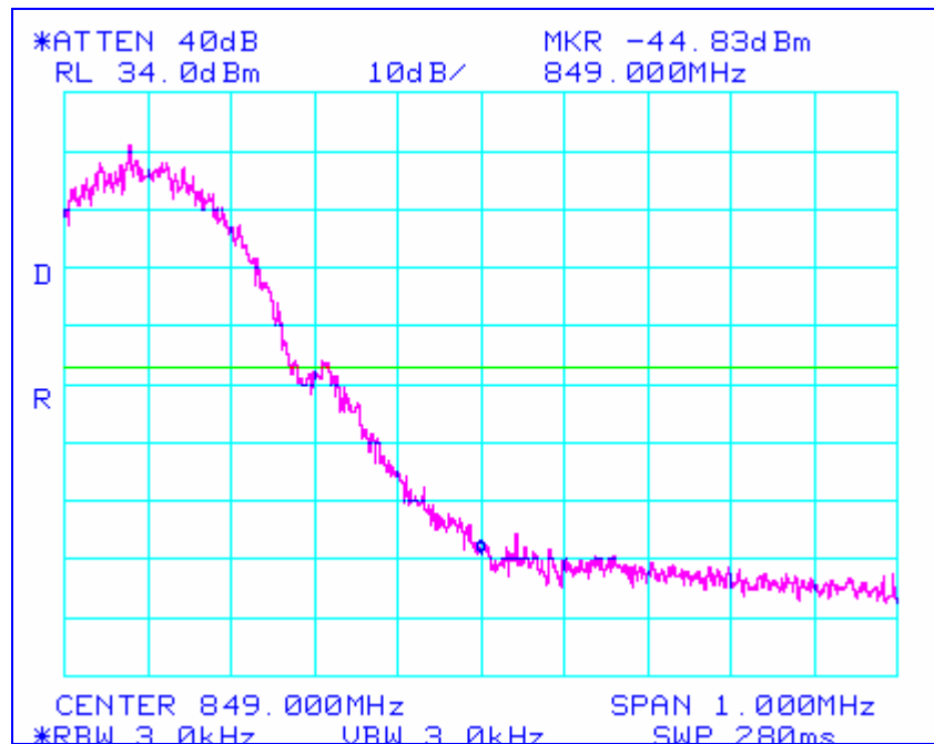
Plot 6 Conducted Spurious Emissions at High Side frequency (block-edge) Test Results
