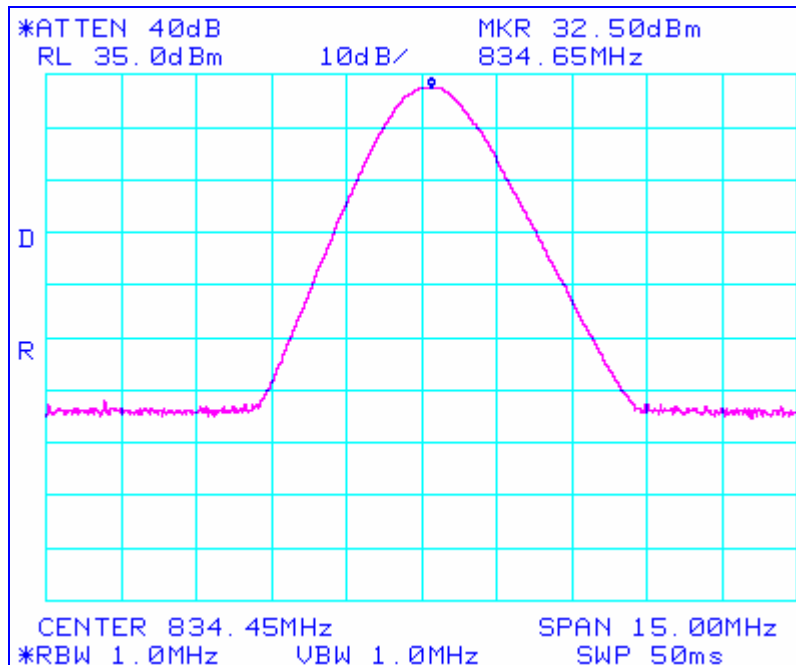
Plot 3 RF Output Power Test Results
