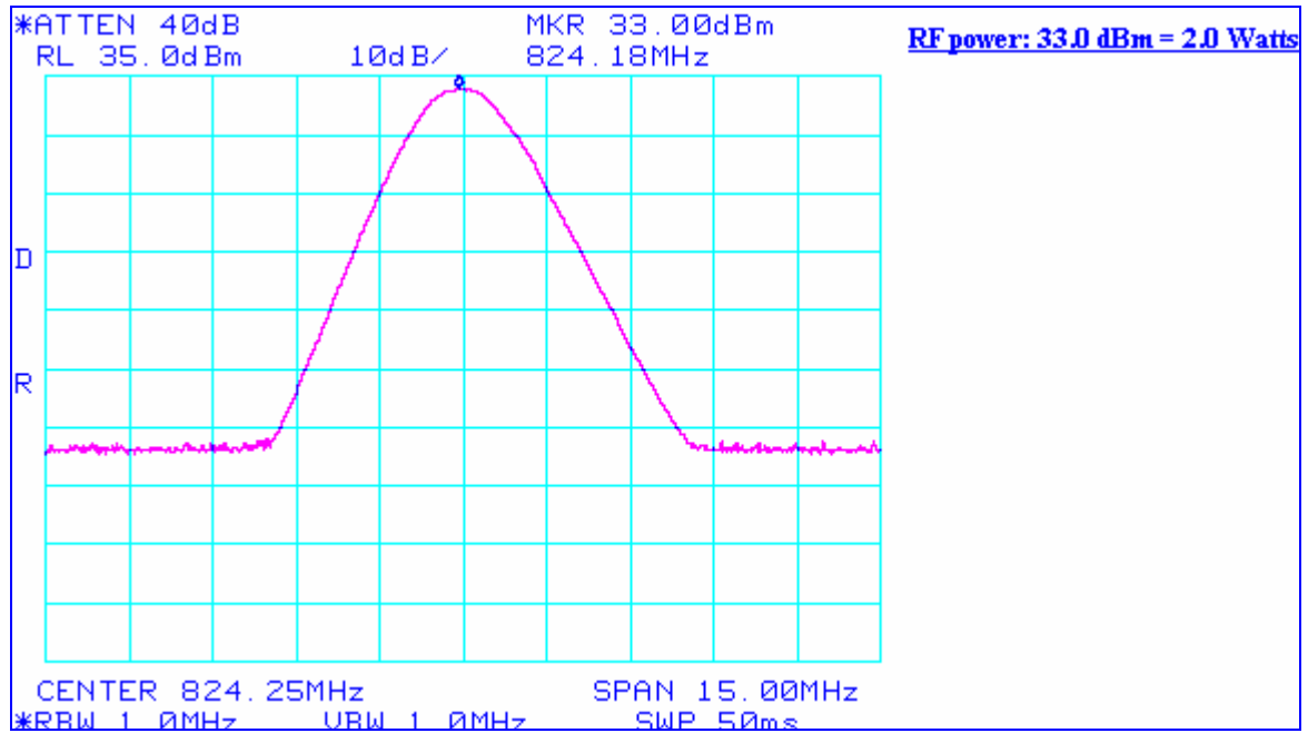
Plot 2 RF Output Power Test Results
