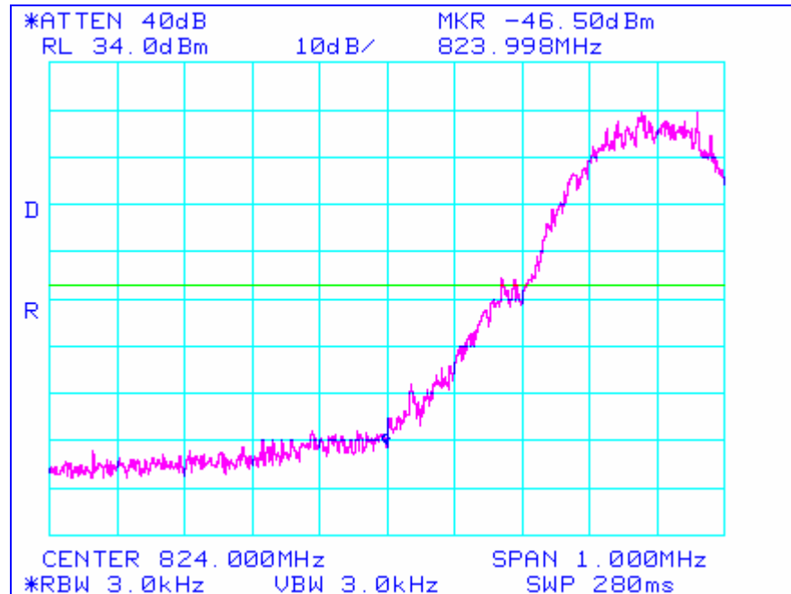
Plot 7 Conducted Spurious Emissions at Low Side frequency (block-edge) Test Results
