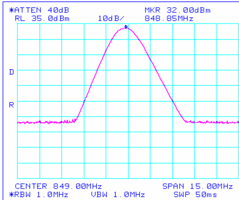
Plot 1 RF Output Power Test Results
