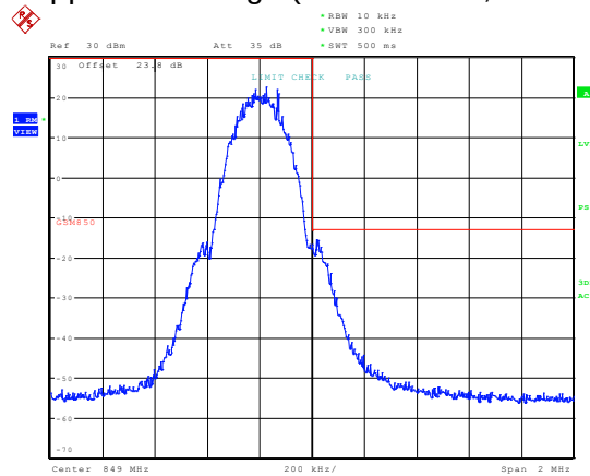
Upper Band Edge (Channel 251, 848.8 MHz)
