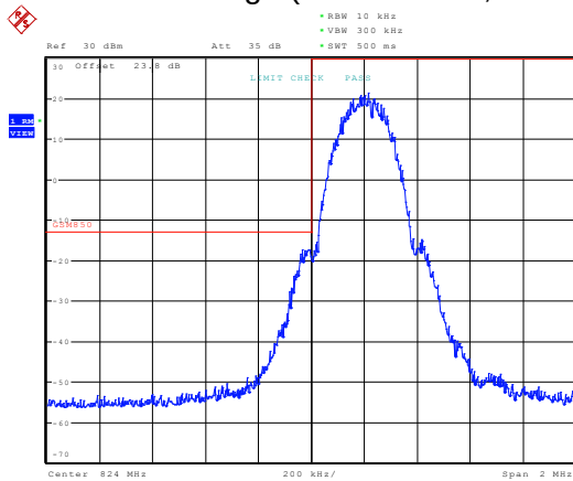
Lower Band Edge (Channel 128, 824.2 MHz)
