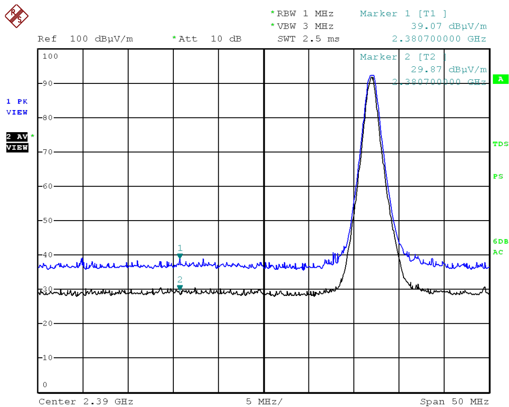
BDR(DH5) Low(Vertical)
