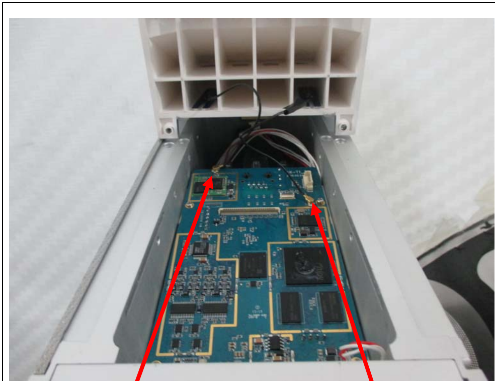
BT Antenna
