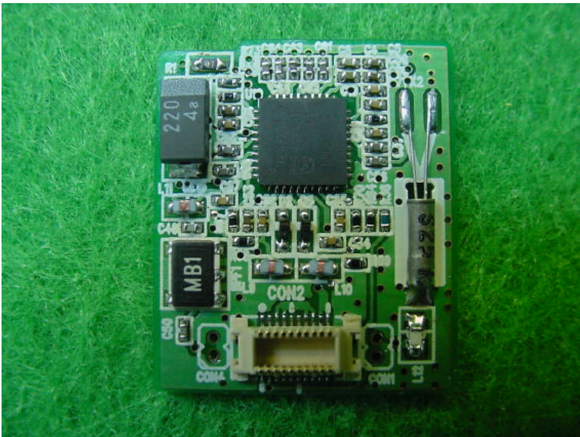
<FRONT SIDE OF TURNER BOARD>
